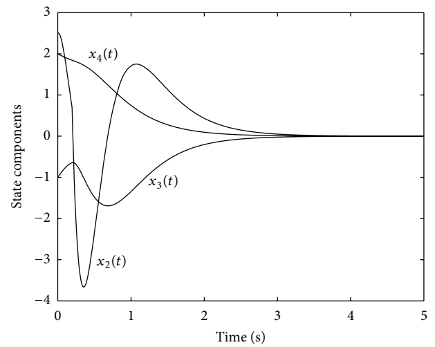
FIGURE 12: Evolution of the state components x_2(t) , x_3(t) , and x_4(t) .
