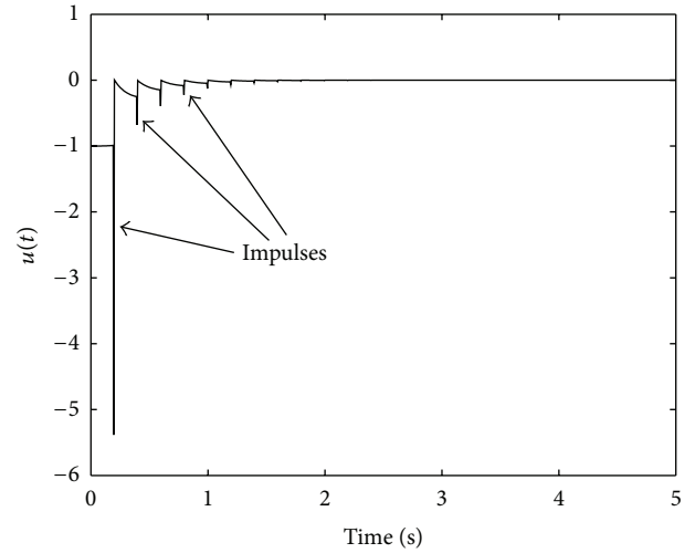
FIGURE 10: Control input with impulses.
