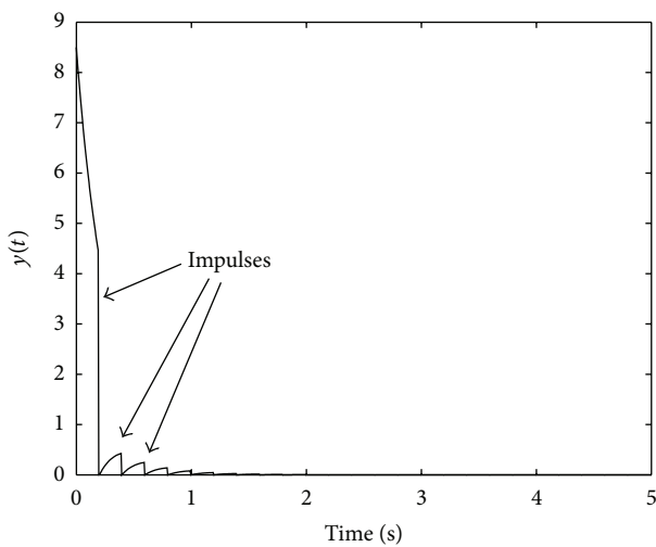
FIGURE 9: System output in the presence of impulses.
