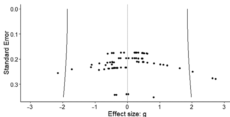
Figure 2. Funnel plot. The fact that effect sizes are symmetrically distributed around the mean effect seems to indicate the absence of publication bias.
