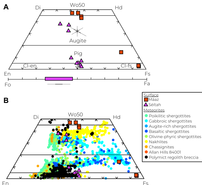
Fig. 5. Pyroxene quadrilateral. (A) Pyroxene compositions observed in Mááz fm (red squares) and Séítah (purple triangles). The range of Mg numbers of Séítah olivines is shown below (see fig. S8). Superposed error bars show mean precision (dark lines) and accuracy (light lines). (B) Comparison with pyroxene composition found in martian meteorites. The Mááz fm contains augite and Fe-rich pyroxenes, similar to basaltic shergottite meteorites, whereas the Séítah fm contains pyroxenes more enriched in Mg, similar to poikilitic and olivine-phyric shergottites. End members and compositions are indicated as follows: Di, diopside; Hd, hedenbergite; Wo50, wollastonite 50%; Pig, pigeonite; Cl-en, clinopyroxene enstatite; Cl-fs, clinopyroxene ferrosilite; En, enstatite; Fs, ferrosilite; Fo, forsterite; Fa, fayalite. Meteorite data in (B) are from references given in reference file S1.
