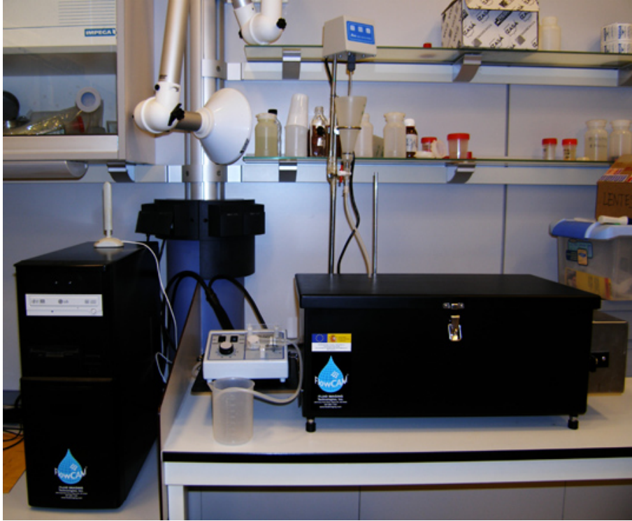
Fig. 1.2. Flowcam, instrument used for phytoplankton digitalization during oceanographic surveys or in laboratories. It is composed of a water plumb, a plastic pipe where the sample goes through and where a digital camera takes several photos per second of the particles in the water sample. Those particles often have sizes inferior to one millimeter. They are later counted and classified using supervised classification methods.
