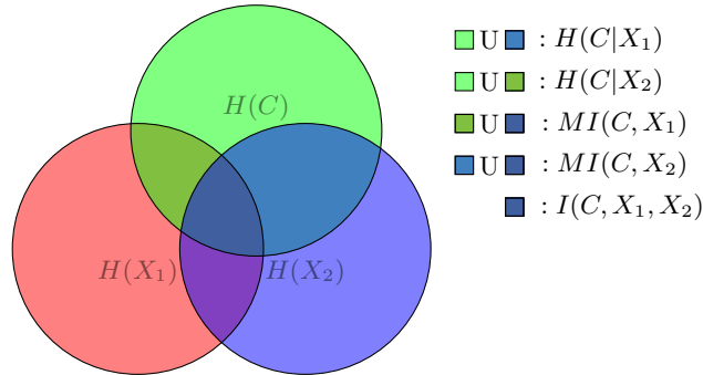
Fig. 3.3. Graphical representation of several information theory uncertainty measures
