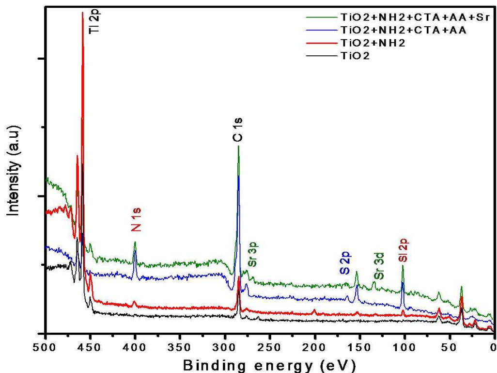
Figure 4.5. XPS Survey scans of PAA polymerization and strontium incorporation. Reaction is followed by XPS for TiO 2 -PAA-35-Sr sample.
