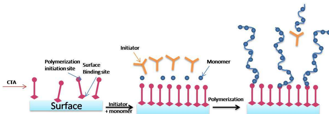
Figure 4.3. Schematic representation of RAFT polymerization on the surface. CTA attaches for the surface from one side while on the other side contains polymerization initiation site. Upon addition of initiator and monomer a polymer brush grows on the surface. Also, free polymer is present in the solution from the initiation of the monomer from the azo-initiator
