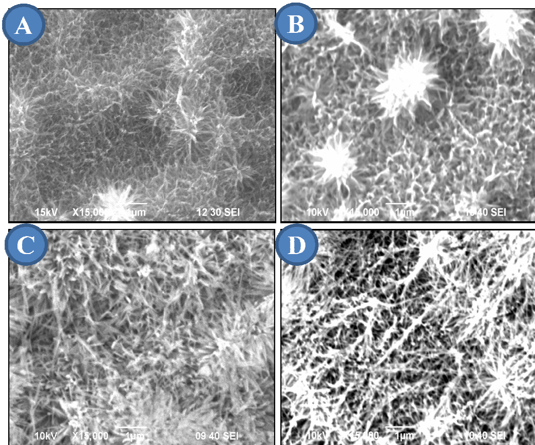
Figure 5.9. SEM images of sandblasted titanium alloys after 3 hours of alkaline treatment at 180 °C with 3 M NaOH solution (A). Titanium alloys after alkaline treatment immersed in 250 mM SrCl 2 solution at different pH values: (B) pH 6, (C) pH 9 and (D) pH 12.
