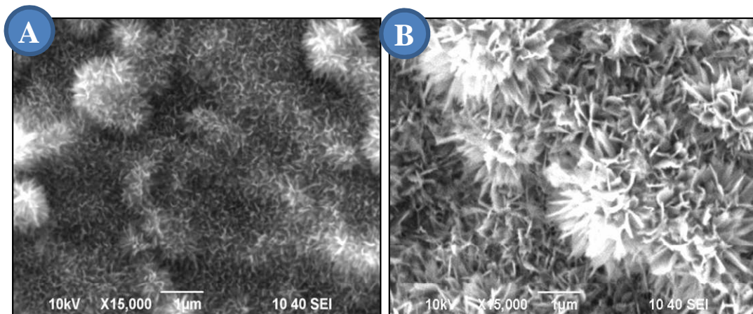
Figure 5.2. Topography of NaOH etched titanium alloys revealed by SEM at a 15000 X magnification. Both samples are sandblasted titanium alloys (Ti-6Al-4V) discs treated for (A) 3 hours and (B) 6 hours at 180°C with 1M NaOH solution.
