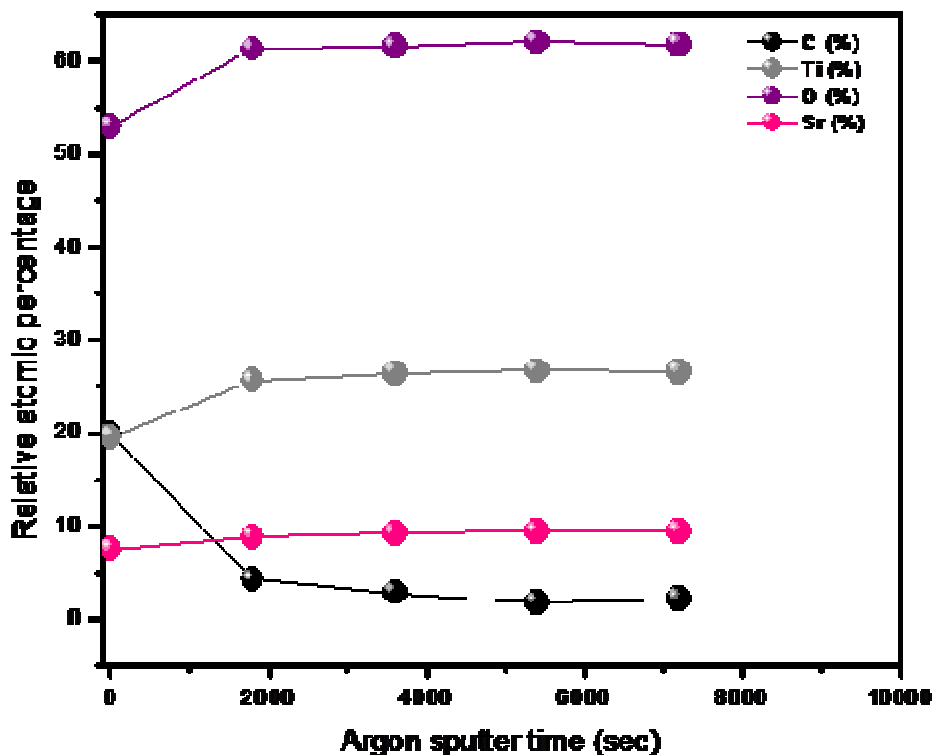
Figure 5.6. XPS depth profile of sandblasted titanium alloy treated with 3M NaOH and immersed in strontium chloride solution. XPS spectra are taken after continuing argon sputtering at 5 times intervals, The initial point corresponding the to the composition of the surface previous to argon sputtering
