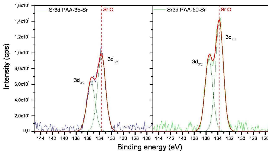
Figure 4.6. XPS detail region of strontium core level, Sr 3d for TiO 2 -PAA-35-Sr (on the left) and TiO 2 -PAA-50-Sr. Intensity scale is in the CPS units and increase in intensity in strontium signal is notable for PAA prepared at higher grafting density (TiO 2 -PAA-50-Sr).
