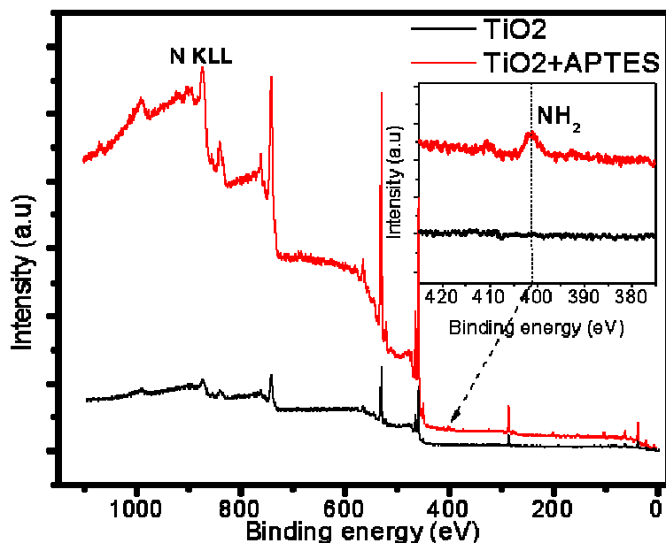
Figure 3.2. XPS survey of APTES on TiO 2 Appearance of the NH 2 peak in the N 1s region after APTES fictionalization (in red).
