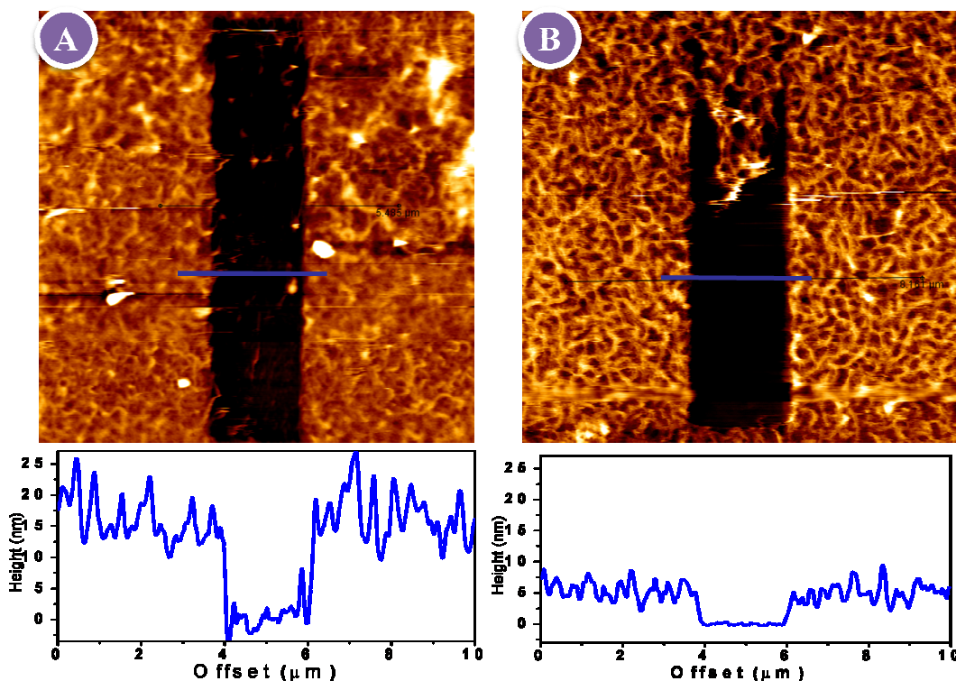
Figure 3.7. AFM topography and height profile. 10 x 10 μm performed by JPK. Topography of 4 layer films prepared as A LbL, in acid medium and B after crosslinking imaged in PBS. Bottom panels are height profiles measured at a cross section indicated in a figures A and B.
