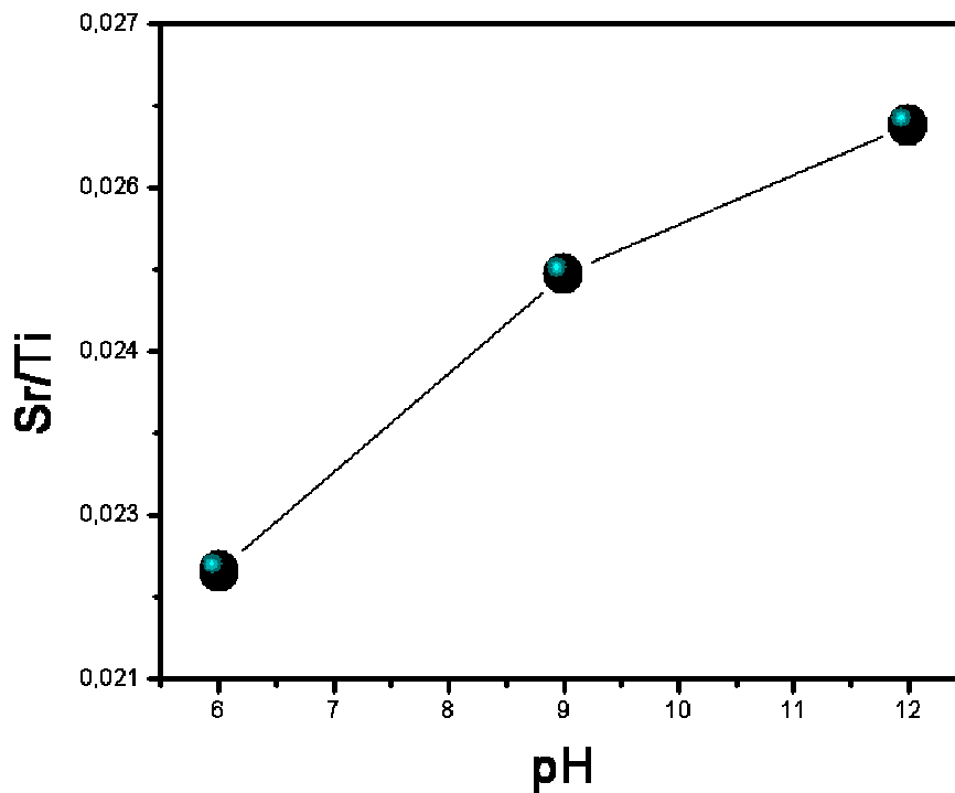
Figure 5.10. Increase in the strontium incorporated into titanium alloy in relation with increase of the SrCl 2 solution pH. Relative amount of strontium is expressed as Sr/Ti ratio resulting from EDX experiments.
