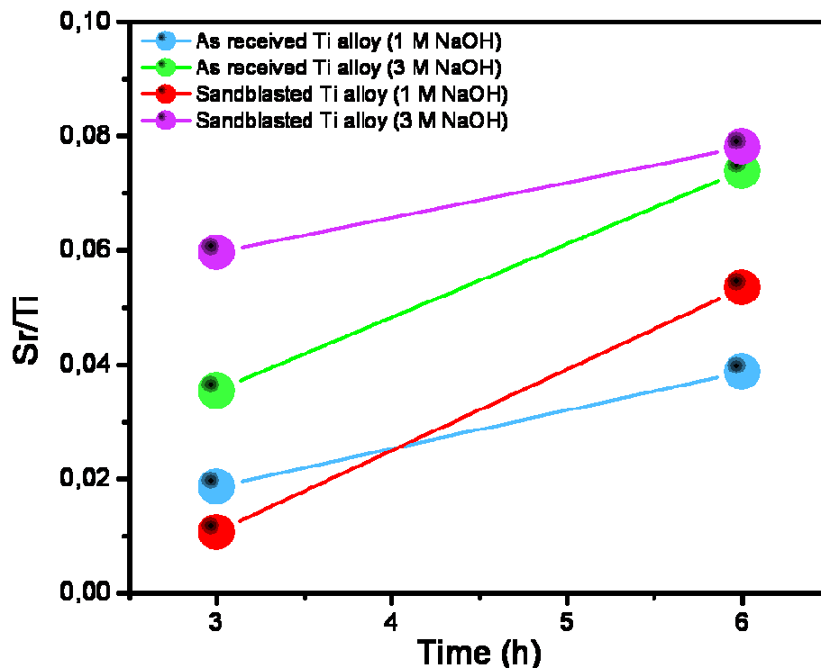
Figure 5.11. Influence of the incubation time with strontium chloride on total Sr incorporated into the as received and sandblasted Ti alloy substrates. pH value of 250 mM \text{SrCl}_2 solution used for this experiment is adjusted to 12. Relative amount of strontium is expressed as Sr/Ti ratio resulting from EDX experiments
