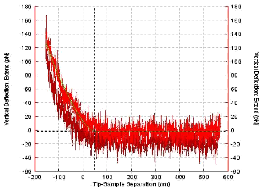
Figure 3.8. AFS typical f-d curve, raw data fit. Bright red is the approach curve and dark red is the retract curve in the cycle.
