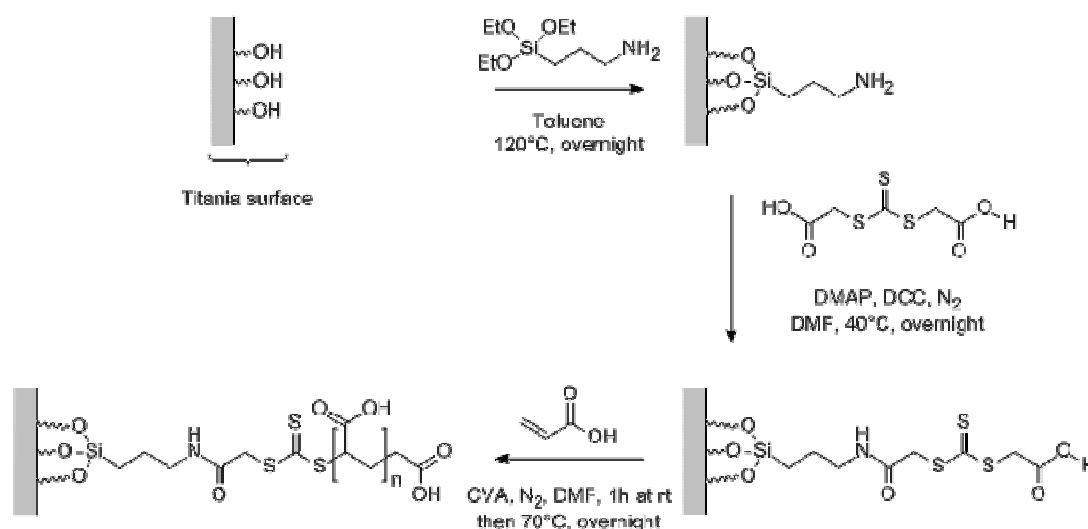
Figure 4.4. Reaction scheme used to prepare a polyacrylic acid brush system on the -NH 2 containing titania surface through RAFT polymerization.
