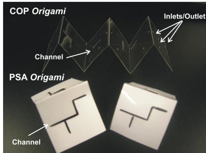
Figure 1: COP and PSA layers after xurography and bending (following the dotted lines) showing the inlets/outlet and channels in detail.
