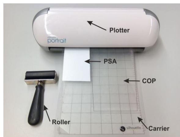
Figure 2: Silhouette Portrait plotter set-up for rapid prototyping and roller.
