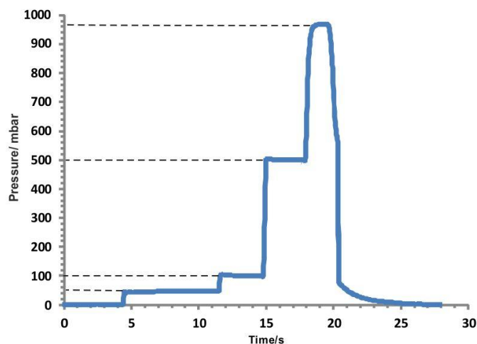
Figure 5: a) Pressures that the micromixer can hold: steps at 50, 100, 500 and 1000 mbar, respectively. The drop of the signal at time 20 s is due to the emptying of the 1 mL reservoir.
