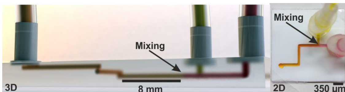
Figure 4: Scheme of the micromixer in 3D view (left) and a 2D view of the micromixer performance when introducing the red and yellow dye solutions at 20 \mu\text{L min}^{-1} (right).
