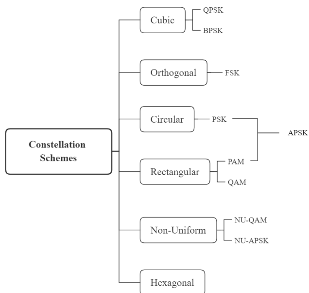
FIGURE 2. Diagram of basic constellations schemes.
