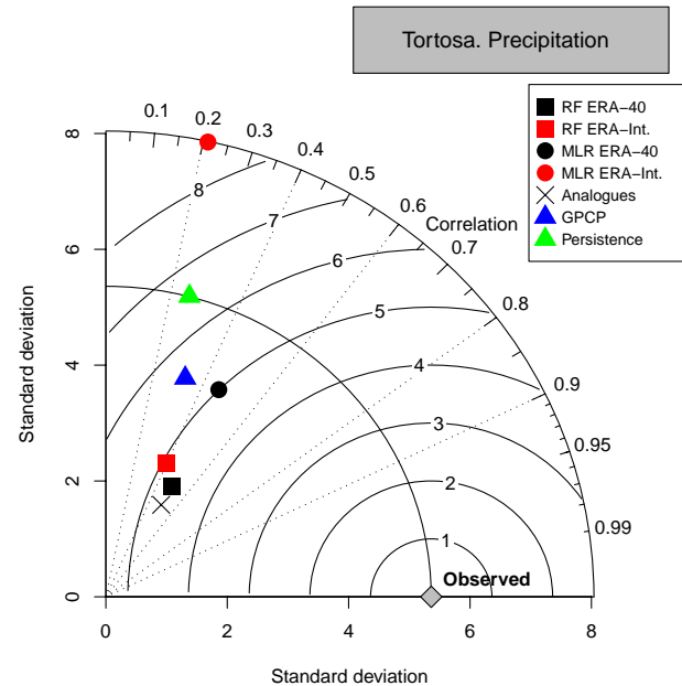
Fig. 7. Taylor's diagram of the models for daily precipitation in Tortosa. 1826 test cases (1997–2001).
