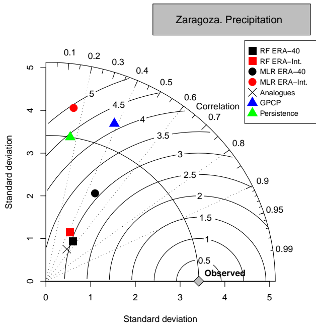
Fig. 4. Taylor's diagram of the models for daily precipitation in Zaragoza. 1826 test cases (1997–2001).
