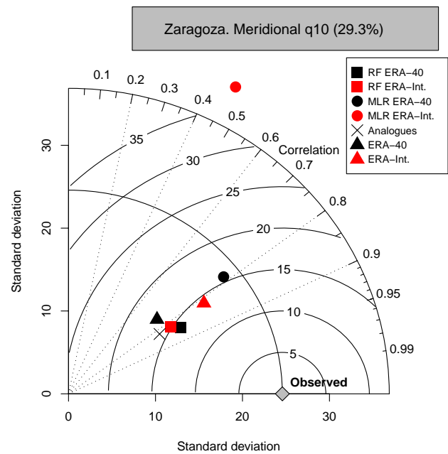
Fig. 3. Taylor's diagram of the models for daily meridional q_{10} in Zaragoza. 1826 test cases (1997–2001). In brackets, percentage of the overall q_{10} variability corresponding to the meridional component.
