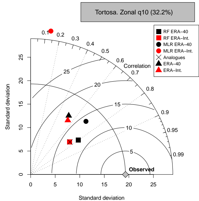
Fig. 5. Taylor's diagram of the models for daily zonal q_{10} in Tortosa. 1826 test cases (1997–2001). In brackets, percentage of the overall q_{10} variability corresponding to the zonal component.
