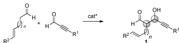
Scheme 1. Catalytic enantioselective approaches to oxygenated 1, \omega -enynes.
