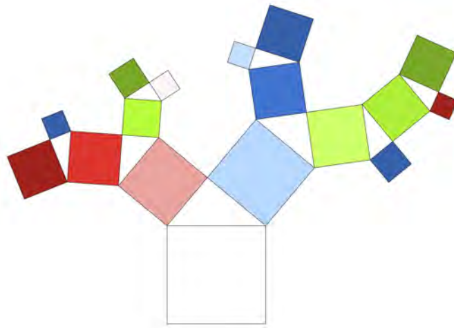
FIGURE 6.17: The pythagorean tree of the decision tree in Figure 6.16 for the three patient groups: ABU (blue), CON (red) and MIG (green). The sides of each triangle relate to the number of observations split by each decision and the node colour denotes the most probable class.
