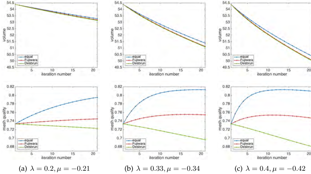
FIGURE 5.5: Volume and mesh quality of the cow geometry after applying the Taubin smoothing with equal, Fujiwara and Desbrun weights at each iteration step for scaling parameters \lambda = 0.2 and \mu = -0.21 (a), \lambda = 0.33 and \mu = -0.34 (b) and \lambda = 0.4 and \mu = -0.42 (c).
