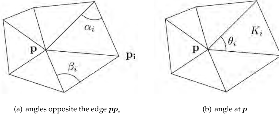
FIGURE 5.2: The notations for the angles opposite the edge \overline{\mathbf{p}\mathbf{p}_i} (a) and for the angle at point \mathbf{p} (b).
