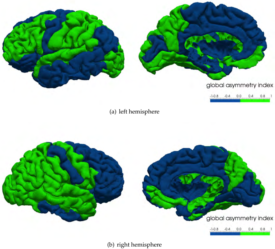
FIGURE 5.16: The global asymmetry index \mathfrak{A}_j^L and \mathfrak{A}_j^R on the left (a) and right hemisphere (b).
