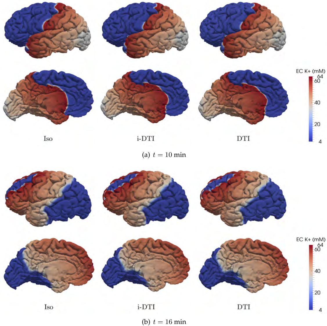
FIGURE 4.19: Lateral and medial view of the CSD wave propagation via the extracellular potassium concentration ( \text{EC K}^+ ) of the left hemisphere at time t = 10 min (a) and t = 16 min (b), for the three different choices of diffusion tensor.
