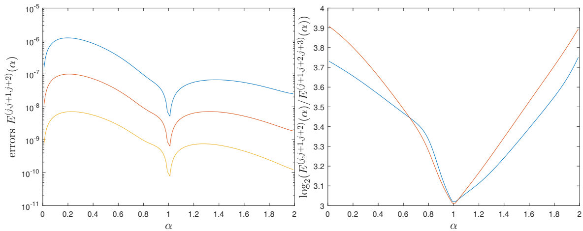
FIGURE 4.13: Left: Errors for [-\Delta^{\alpha/2}]^{(j,j+1,j+2)}e^{i2s} . Right: Convergence rate. We have used (4.46) and fast convolution applying Richardson extrapolation twice, taking \alpha \in \{0.01, \dots, 0.99\} \cup \{1.01, \dots, 1.99\} , N = 128 , j = 1, \dots, 3 .
