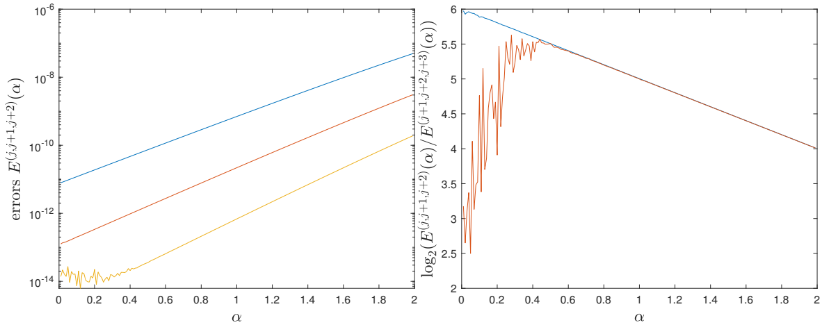
FIGURE 4.16: Left: Errors for [-\Delta^{\alpha/2}]^{(j,j+1,j+2)} e^{-x^2} . Right: Convergence rate. We have used (4.46) and fast convolution applying Richardson extrapolation twice, taking \alpha \in \{0.01, \dots, 0.99\} \cup \{1.01, \dots, 1.99\} , N = 128 , j = 1, \dots, 3 .
