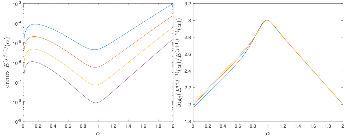
FIGURE 4.12: Left: Errors for [-\Delta^{\alpha/2}]^{(j,j+1)}e^{i2s} . Right: Convergence rate. We have used (4.46) and fast convolution applying Richardson extrapolation once, taking \alpha \in \{0.01, \dots, 0.99\} \cup \{1.01, \dots, 1.99\} , N = 128 , j = 1, \dots, 4 .
