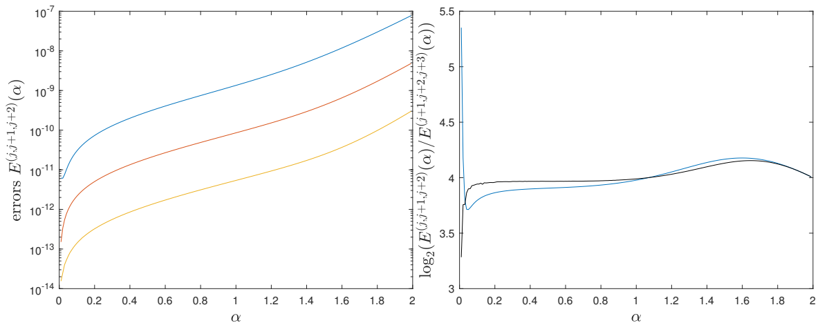
FIGURE 4.10: Left: Errors for [(-\Delta)^{\alpha/2}]^{(j,j+1,j+2)} e^{-x^2} . Right: Convergence rate. We have used (4.36) and fast convolution applying Richardson extrapolation twice, taking \alpha \in \{0.01, \dots, 0.99\} \cup \{1.01, \dots, 1.99\} , N = 128 , j = 1, \dots, 3 .
