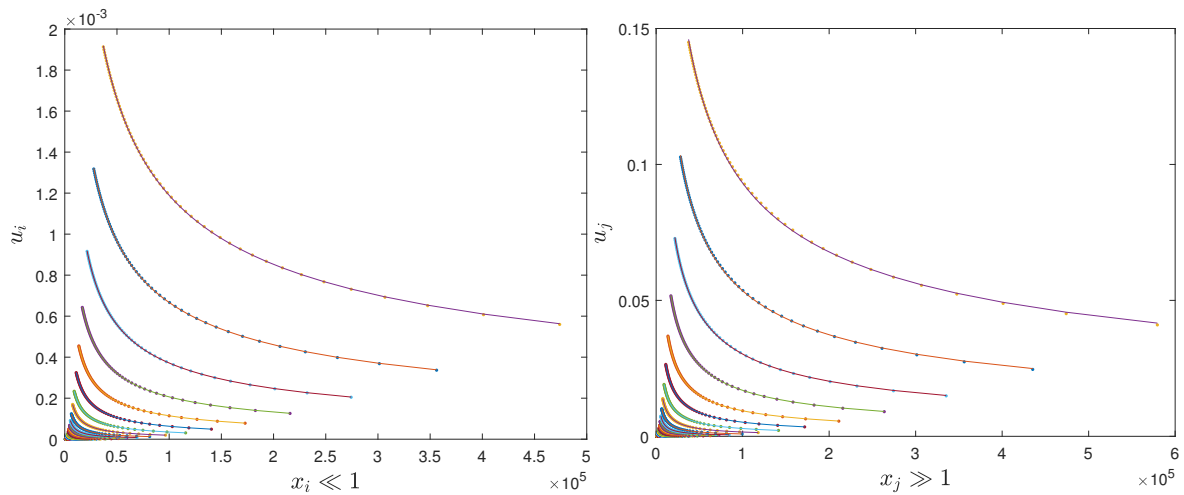
FIGURE 2.6: \alpha = 0.5, 0.55, \dots, 1.95 , L = 10^3/\alpha^3 , \Delta t = 0.01 and N = 1024 . Left: least-square fitting for u_i \rightarrow 1 against x_i \ll 1 . Right: least-square fitting for u_j \rightarrow 0 against x_j \gg 1 .
