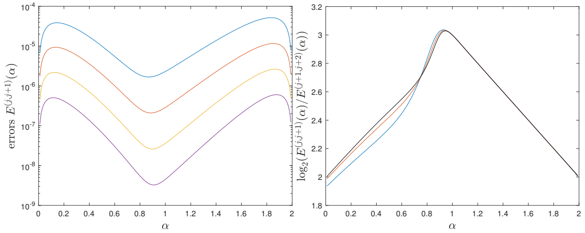
FIGURE 4.6: Left: Errors for [-\Delta^{\alpha/2}]^{(j,j+1)}e^{i2s} . Right: Convergence rate. We have used (4.36) and fast convolution applying Richardson extrapolation once, taking \alpha \in \{0.01, \dots, 0.99\} \cup \{1.01, \dots, 1.99\} , N = 128 , j = 1, \dots, 4 .
