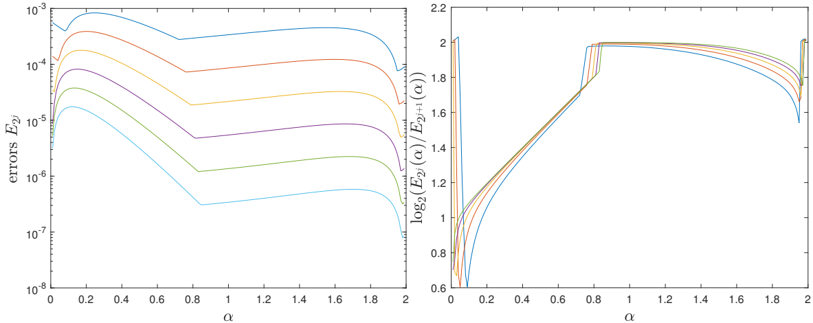
FIGURE 4.3: Left: Errors for (-\Delta)^{\alpha/2} e^{i2s} . Right: Convergence rate. We have applied the fast convolution scheme, using a regular function as the integrand, taking \alpha \in \{0.01, \dots, 0.99\} \cup \{1.01, \dots, 1.99\} , and N = 2^j nodes, with j = 7, 8, \dots, 12 .
