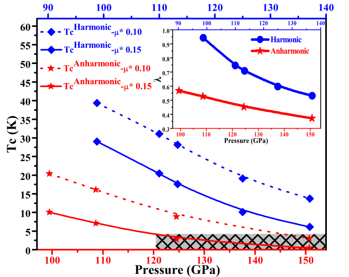
Figure 4: (Color online) Superconducting critical temperature T_c and electron-phonon coupling constant \lambda (inset) as a function of pressure in the harmonic approximation (blue lines) and considering anharmonic effects (red lines). Note that a different pressure scale is used for the harmonic and anharmonic calculations, which includes quantum effects for the latter but not the former. Harmonic and anharmonic results aligned vertically are calculated with the same lattice parameter. T_c calculated with \mu^* = 0.10 and 0.15 is plotted with dotted lines and solid lines respectively. The grey shadow box marks the pressure region in which no superconductivity was found experimentally above 4 K[32].
