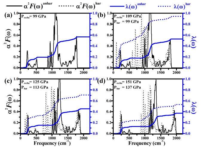
Figure 5: Anharmonic spectral function \alpha^2F(\omega) (black solid lines) and integrated electron-phonon coupling constant \lambda(\omega) (blue solid lines) at four different quantum pressures: (a) 99 GPa, (b) 109 GPa, (c) 125 GPa, and (d) 151 GPa, respectively. The harmonic results obtained are also shown with dotted lines using the same colors for comparison at three different classical pressures: (b) 99 GPa, (c) 113 GPa and (d) 137 GPa. The harmonic and anharmonic results in each panel are obtained with the same lattice parameter.
