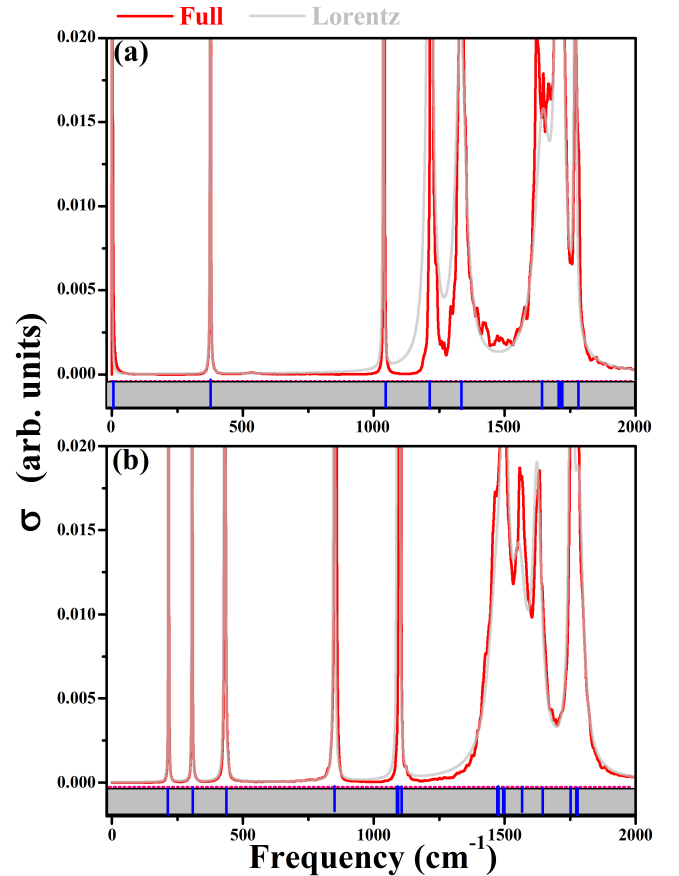
Figure 3: (Color online) Phonon spectral function \sigma(\mathbf{q}, \Omega) of AlH 3 at 99 GPa (pressure calculated with anharmonic quantum effects), at (a) the \Gamma point and (b) the X point. The red line indicates the result obtained keeping the full energy dependence on the self-energy and the grey line indicates the spectrum calculated in the Lorentzian approximation[41, 46]. The centers of these Lorentzians define the anharmonic phonon frequencies. They are indicated with the blue short vertical lines in the lower panel with grey background.
