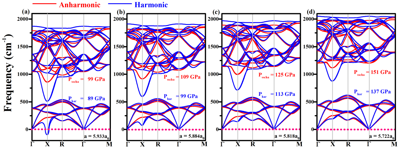
Figure 2: (Color online) Comparison between the harmonic (blue solid lines) and anharmonic (red solid lines) phonon spectra of the cubic high-symmetry Pm\bar{3}n phase of \text{AlH}_3 for different lattice parameters. The anharmonic spectra are obtained from \mathbf{D}^{(F)} and correspond to the static limit of the SSCHA dynamical theory. The pressure calculated classically (harmonic calculation) and with quantum effects (anharmonic calculation) is marked in each case. The region of positive and negative frequencies, which represent imaginary frequencies, are separated with a pink dotted line.
