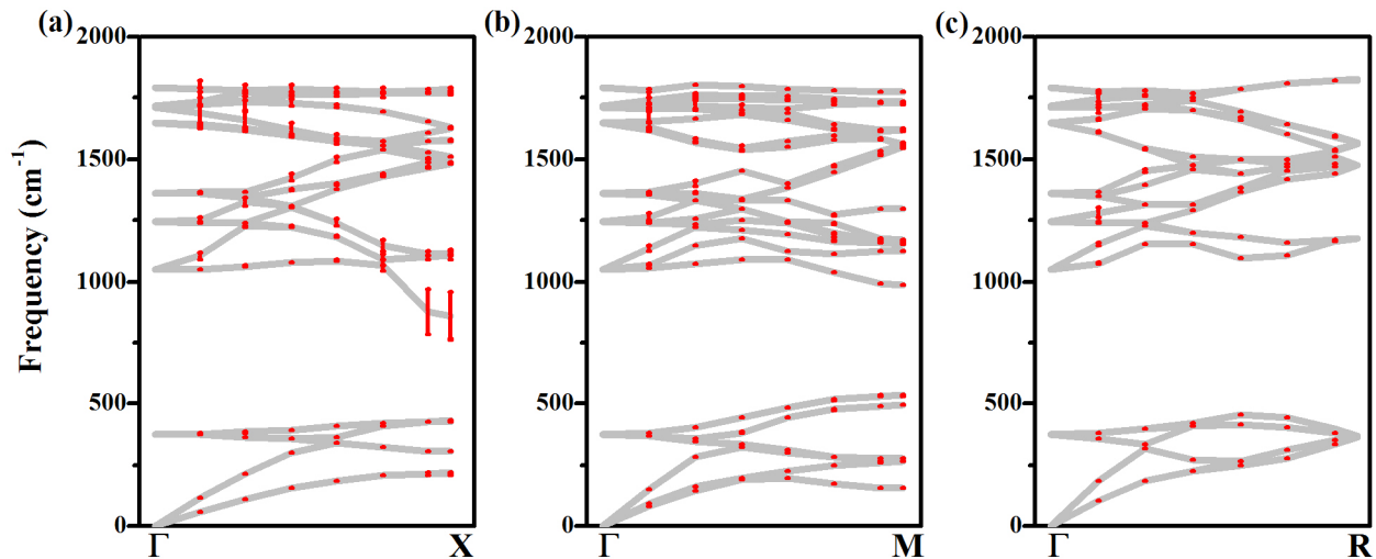
Figure 7: (Color online) The linewidth associated to the electron-phonon interaction calculated with the spectra obtained from D^{(\text{F})} for the cubic high-symmetry Pm\bar{3}n phase of \text{AlH}_3 at 99 GPa (pressure calculated including quantum effects). (a) \Gamma - X path, (b) \Gamma - M path, and (c) \Gamma - R path. The phonon linewidth is indicated by the size of the red error bars.
