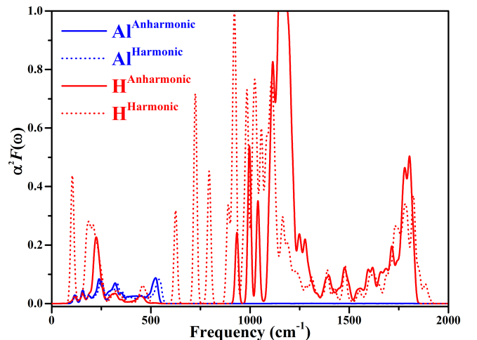
Figure 6: The projected \alpha^2F(\omega) onto Al and H at the harmonic and anharmonic calculated with the same lattice parameter 5.884 a_0 , which corresponds in the quantum anharmonic case to 109 GPa. The harmonic results are shown with dotted lines using same colors for comparison.
