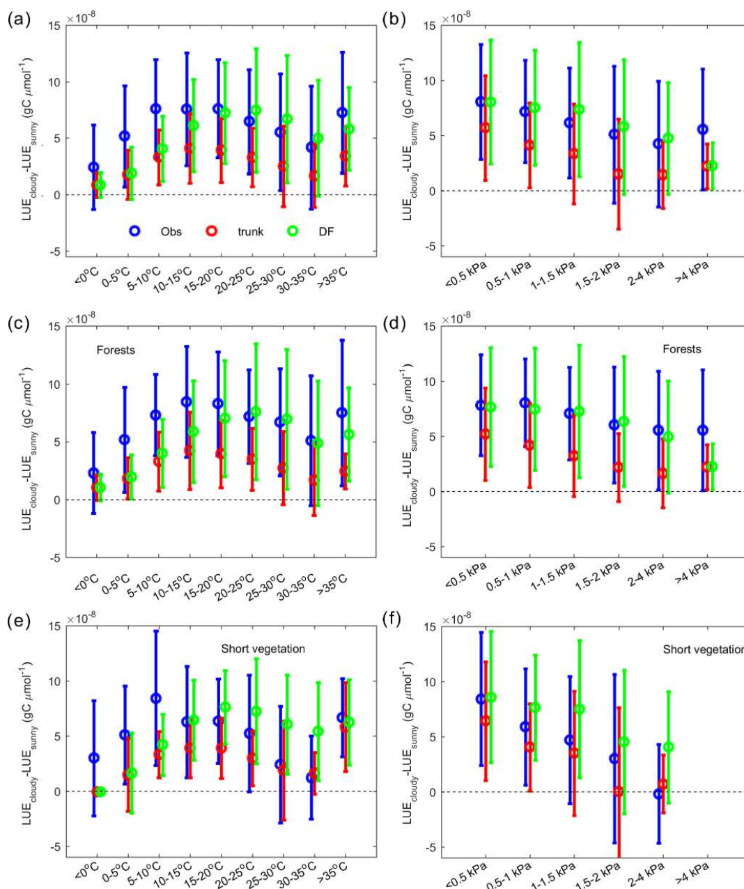
Figure 8. The dependence of the LUE difference between cloudy and sunny conditions on climate factors. In the observations (blue), ORCHIDEE trunk (red) and ORCHIDEE_DF (green), the average and error bars indicate statistics of site-level means. (a) The dependence of the LUE difference on temperature. (b) The dependence of the LUE difference on VPD. Panels (c) and (e) are the same as panel (a) but for forest sites and short vegetation (grasslands and croplands) sites only. Panels (d) and (f) are the same as panel (b) but for forest sites and short vegetation sites only.
