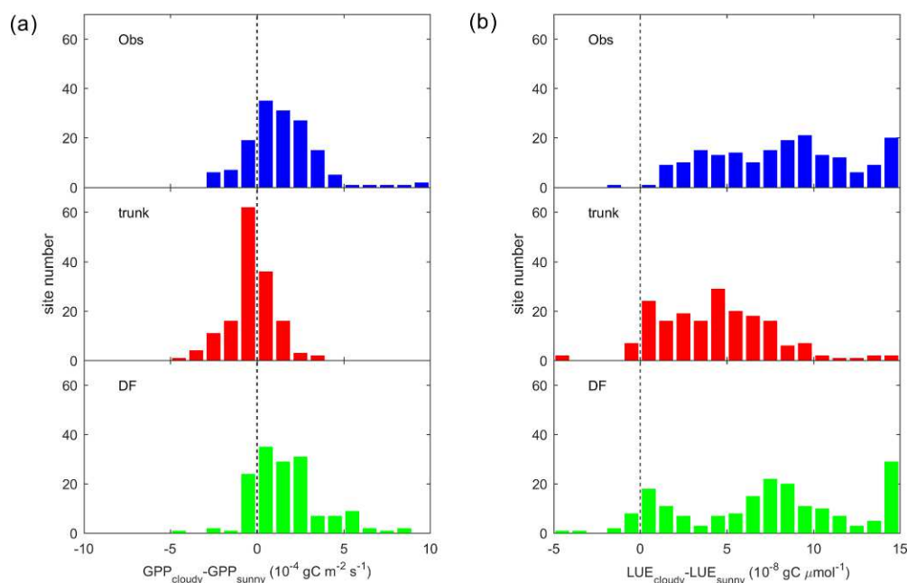
Figure 6. Site distribution of (a) the GPP difference between cloudy (diffuse light fraction >0.8) and sunny (diffuse light fraction <0.4) conditions. Panel (b) is the same as panel (a) but for the LUE. The sunny and cloudy time steps are sampled at equal light levels.
