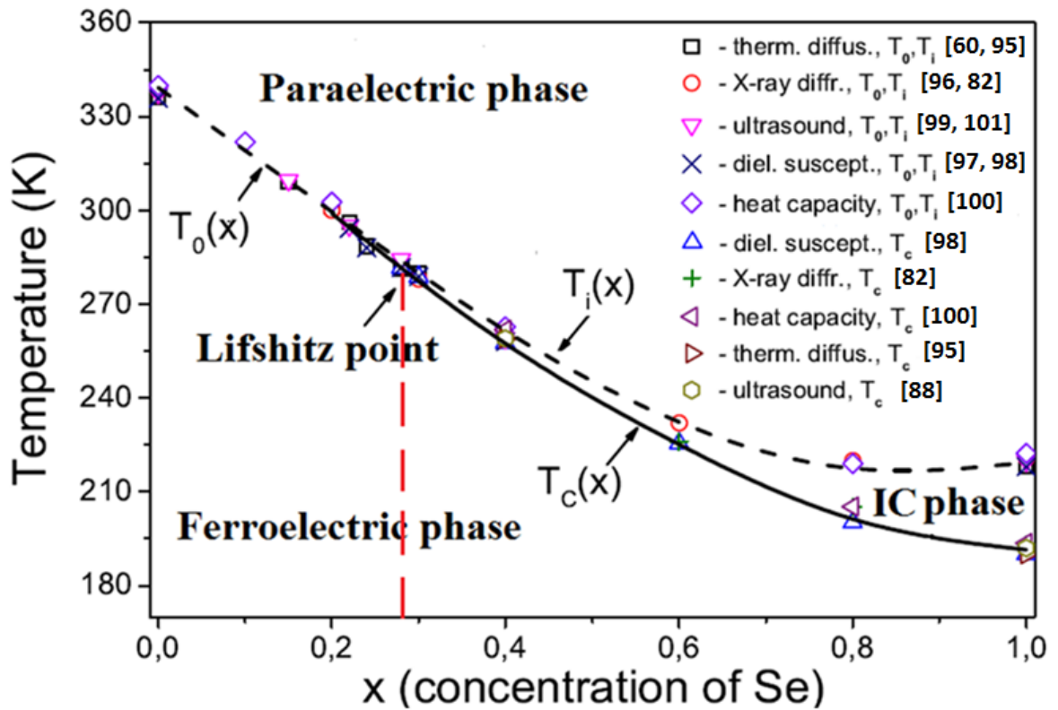
Fig. 3.8. Phase diagram of \text{Sn}_2\text{P}_2(\text{S}_{1-x}\text{Se}_x)_6 crystals. T_0(x) at x < 0.28 and T_i(x) at x > 0.28 are the second order paraelectric-ferroelectric and paraelectric-IC transitions, respectively (dashed line). T_c(x) is the first-order lock-in IC-ferroelectric transition at x > 0.28 (solid line) [101].
