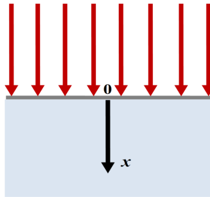
Fig. 1.2. The opaque, semi-infinite material illuminated by a modulated light beam.
