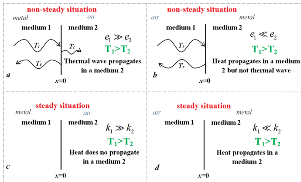
Fig.1.5. Thermal wave propagation through the two media.
