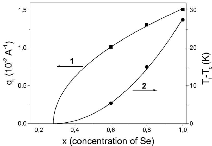
Fig. 3.9. The concentration dependences of the modulation wave number q_i (1) along the T_i(x) line and the temperature width T_i - T_c (2) in \text{Sn}_2\text{P}_2(\text{S}_{1-x}\text{Se}_x)_6 ferroelectrics [101].
