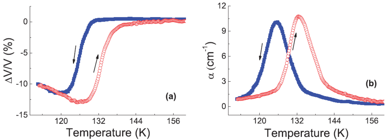
Fig. 3.21. Ultrasound velocity (a) and attenuation (d) for (\text{Sn}_{0.55}\text{Pb}_{0.45})_2\text{P}_2\text{S}_6 ferroelectric performed at cooling (blue) and heating (red) runs [107].
