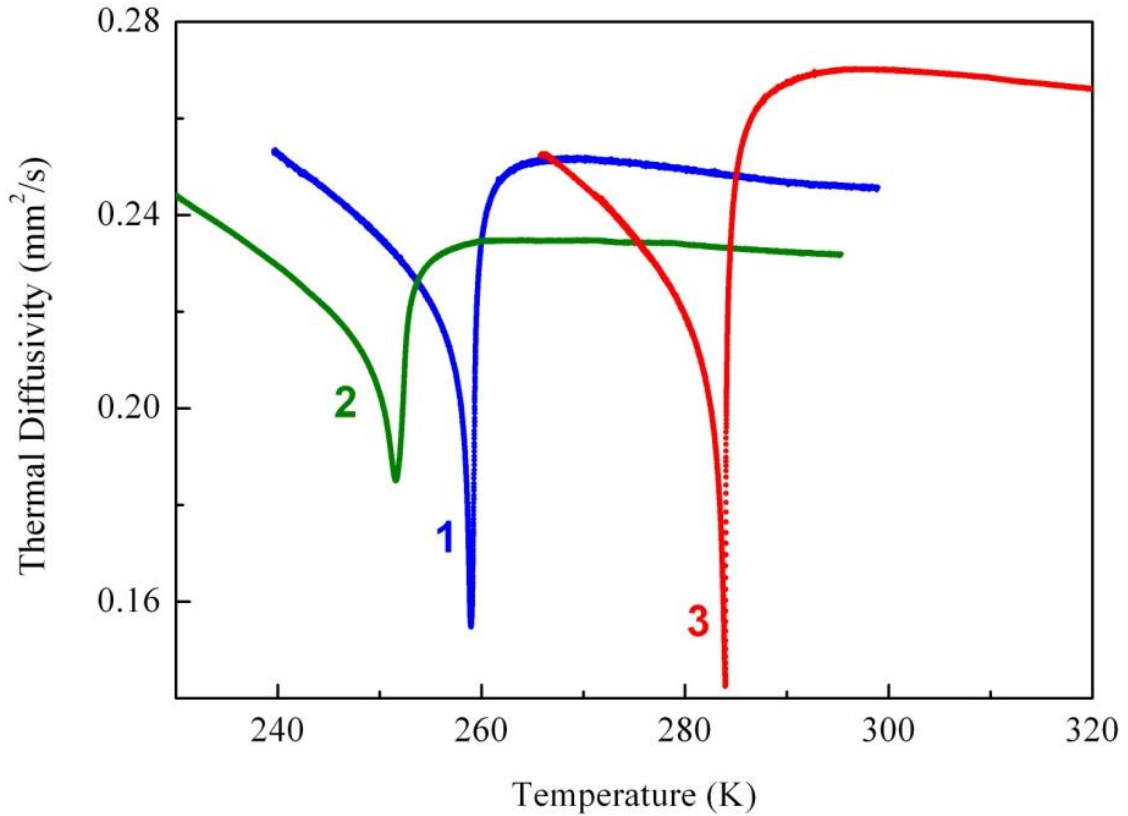
Fig. 8.2. Thermal diffusivity as a function of temperature in the vicinity of T_C for \text{Sn}_2\text{P}_2(\text{S}_{0.72}\text{Se}_{0.28})_6 doped with 5% Pb, 8% Pb and, 5% Ge (curves 1, 2 and 3, respectively).
