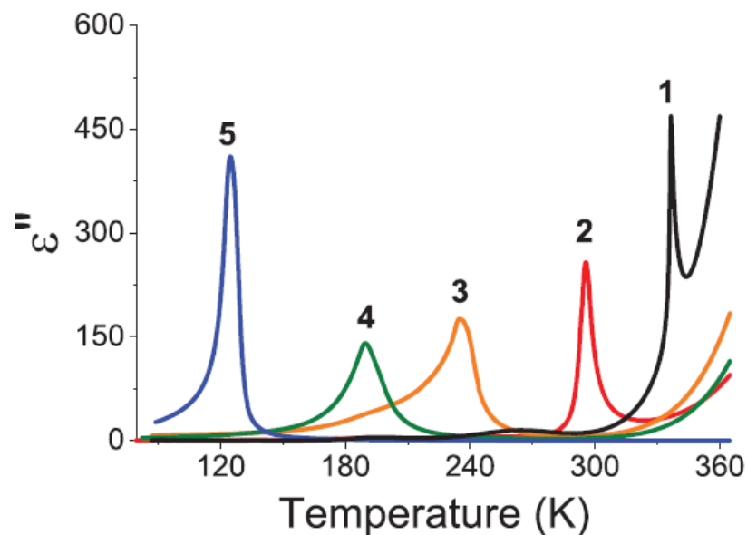
Fig. 3.18. Imaginary part of dielectric susceptibility at 100kHz in cooling runs for (\text{Sn}_{1-y}\text{Pb}_y)_2\text{P}_2\text{S}_6 ferroelectrics: 1 – y=0 ; 2 – y=0.1 ; 3 – y=0.2 ; 4 – y=0.3 ; 5 – y=0.45 [107].
