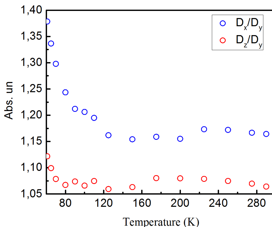
Fig. 5.6. Normalized thermal diffusivity as a function of temperature for x-cut (blue circles) and z-cuts (red circles) of \text{Pb}_2\text{P}_2\text{S}_6 .
