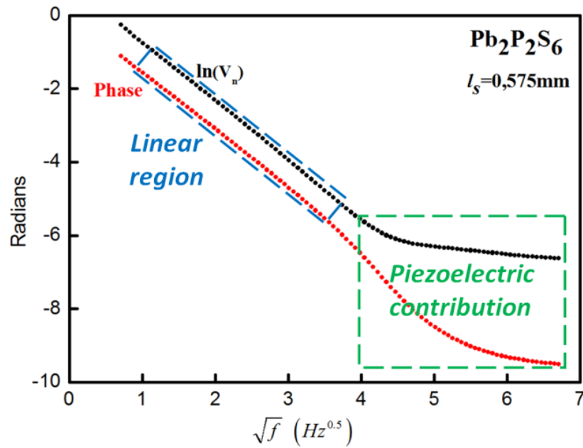
Fig. 2.6. Frequencies scan at room temperature for paraelectric crystal \text{Pb}_2\text{P}_2\text{S}_6 .
