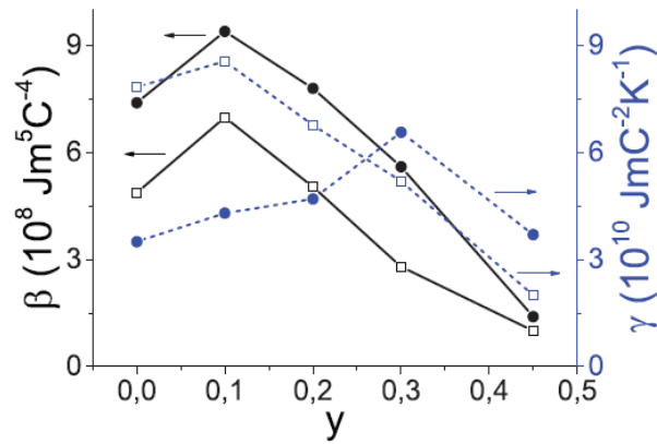
Fig. 3.22. Concentration dependencies of coefficients \beta and \gamma in Landau thermodynamic potential. Solid symbols represent hypersound data analysis, open symbols – ultrasound. [107].
