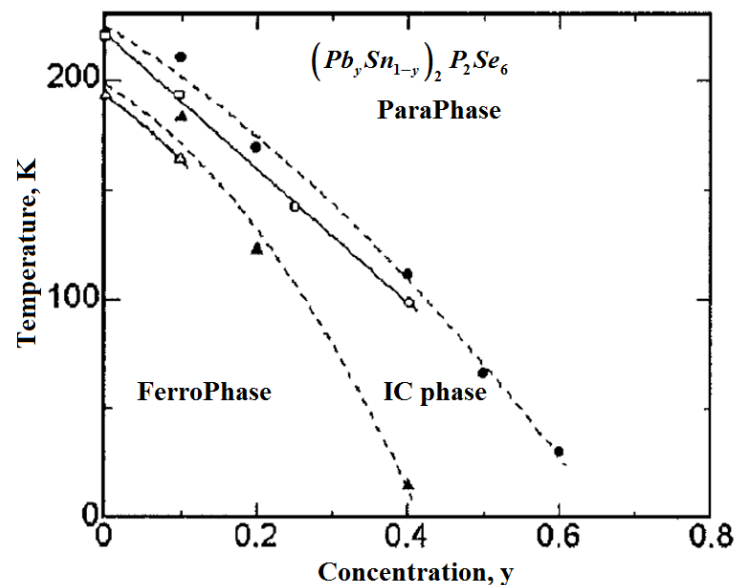
Fig. 3.23. Phase transitions temperatures as a function of lead concentration. Solid symbols represent high-temperature Paraelectric-IC phase transitions (second order) and empty symbols the lock-in IC-ferroelectric phase transitions, which are first order. Circles correspond to data [110] and triangles to [94].
