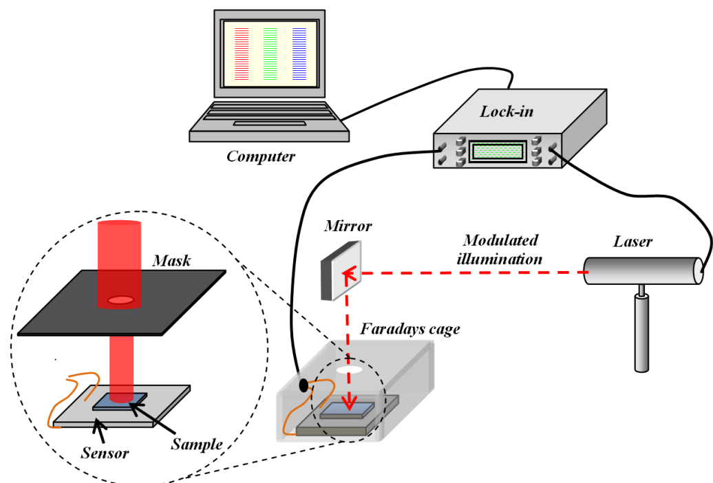
Fig. 2.5. Scheme to perform frequency scans in BPPE configuration at room temperature.
