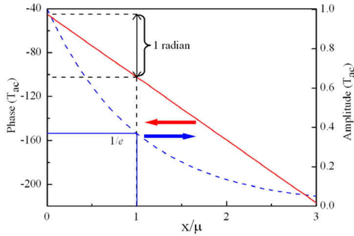
Fig.1.3. The normalized phase and amplitude of the time-dependent component T_{ac} as a function of the reduced depth x/\mu .
