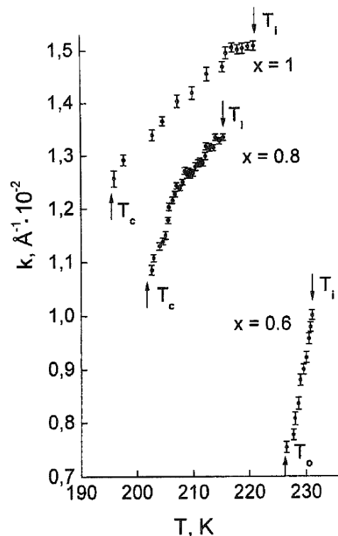
Fig. 3.5. Temperature behavior of the modulation wave vector for \text{Sn}_2\text{P}_2(\text{S}_{1-x}\text{Se}_x)_6 crystals [3].
