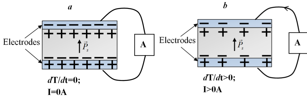
Fig. 2.1. Schematic illustration a nature of pyroelectricity.
