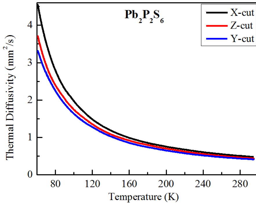
Fig.5.5. Thermal diffusivity as a function of temperature for \text{Pb}_2\text{P}_2\text{S}_6 crystal along its principal crystallographic directions [205].
