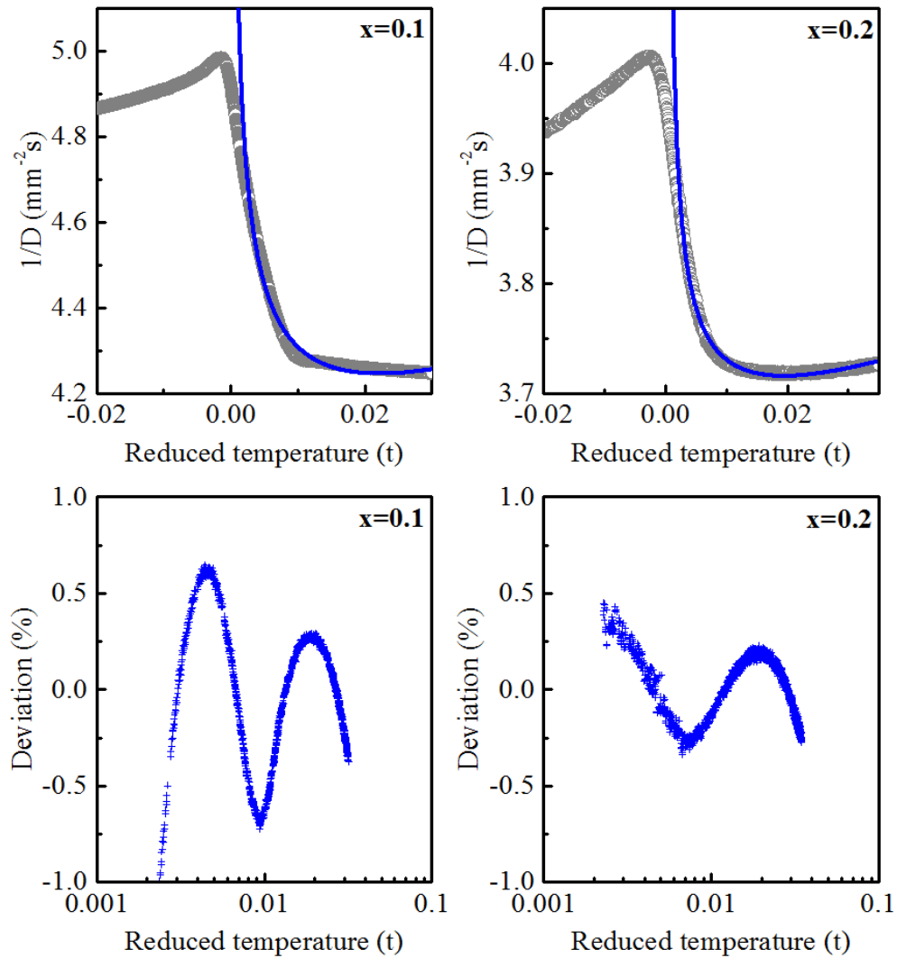
Fig. 5.9. Above: Experimental data for the inverse of thermal diffusivity (grey circles) for (\text{Pb}_x\text{Sn}_{1-x})_2\text{P}_2\text{S}_6 crystals together with their fits to eq.5.5 (blue lines). Below: Deviation plots corresponding to the fittings, presented in percentage [205].
