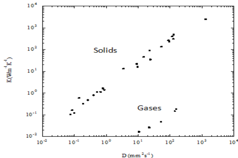
Fig. 1.9. Relation between thermal conductivity and diffusivity in solids and gases [19].
