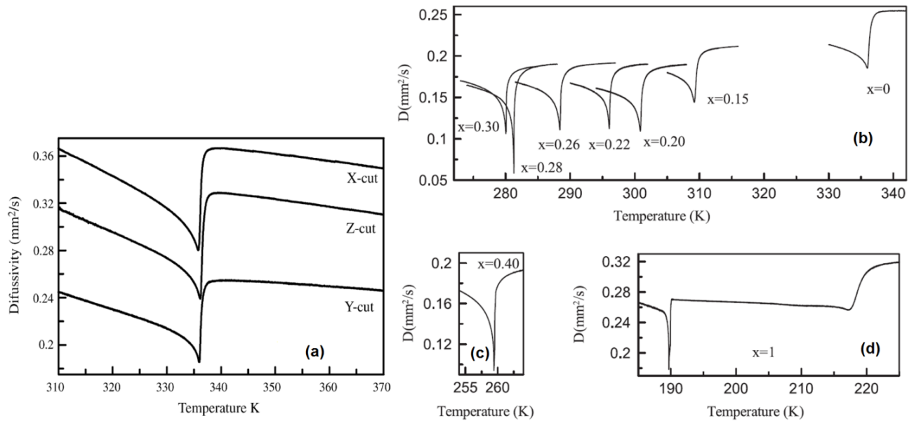
Fig.3.29. Temperature evolution of thermal diffusivity for \text{Sn}_2\text{P}_2\text{S}_6 crystal in different crystallographic directions (a), and for \text{Sn}_2\text{P}_2(\text{S}_{1-x}\text{Se}_x)_6 in [010] direction (b, c, d) [60, 95].
