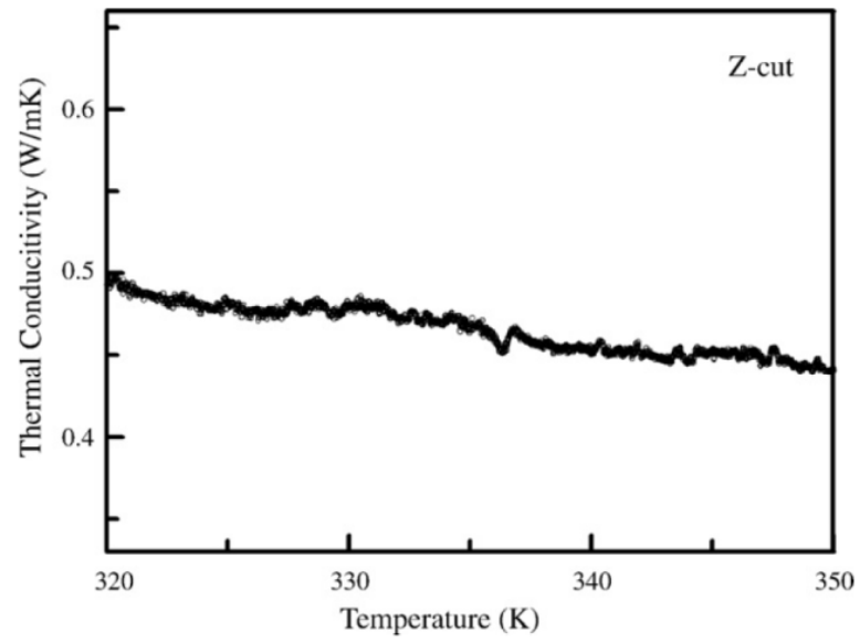
Fig. 3.32. Thermal conductivity of \text{Sn}_2\text{P}_2\text{S}_6 crystal in [001] direction [95].
