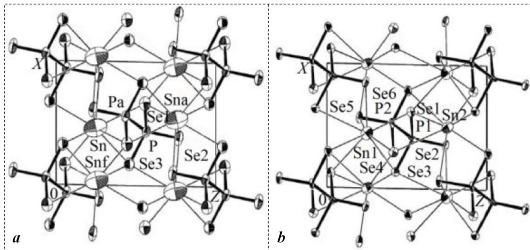
Fig. 3.2. Crystalline structure of \text{Sn}_2\text{P}_2\text{Se}_6 (projection onto (010)): a – paraelectric phase (293K); b – ferroelectric phase (150K) [83].
