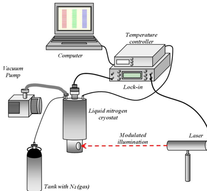
Fig. 2.8. Scheme of experimental setup for measurements as a function of temperature in the range 77-400 K. Laser , He-Ne. Temperature Controller : Oxford Instruments Mod ITC 502. Lock-in . EG & G Instruments, DSP Mod 7265. Cryostat : Optistat DN .
