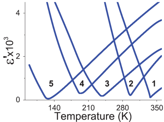
Fig. 3.19. The reciprocal real part of dielectric susceptibility at 100kHz on cooling runs for (\text{Sn}_{1-y}\text{Pb}_y)_2\text{P}_2\text{S}_6 ferroelectrics: 1 – y=0 ; 2 – y=0.1 ; 3 – y=0.2 ; 4 – y=0.3 ; 5 – y=0.45 [107].
