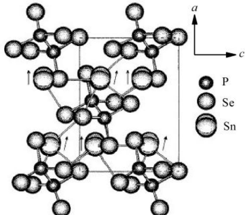
Fig. 3.3. Compared structures of \text{Sn}_2\text{P}_2\text{Se}_6 in the paraelectric and in the ferroelectric phases. Arrows show the \text{Sn}^{2+} cations displacements at the transition to the ferroelectric phase [78, 84].
