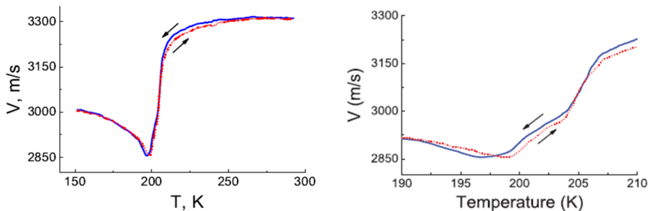
Fig. 3.20. Ultrasound velocity data at cooling (blue) and (heating) runs performed for (\text{Sn}_{0.7}\text{Pb}_{0.3})_2\text{P}_2\text{S}_6 [107].
