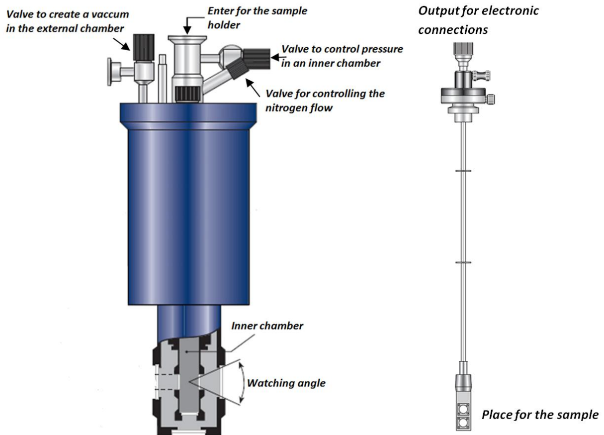
Fig. 2.9. Scheme of a cryostat for investigations between 77-400K.
