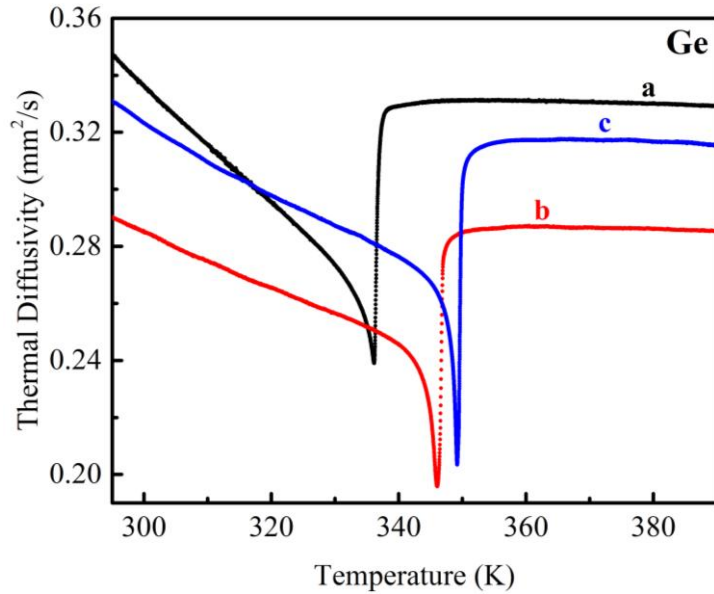
Fig. 7.1. Thermal diffusivity in the (001) direction as a function of temperature for \text{Sn}_2\text{P}_2\text{S}_6 doped with Ge: (a) pure \text{Sn}_2\text{P}_2\text{S}_6 [95]; (b) \text{Sn}_2\text{P}_2\text{S}_6+3\% \text{Ge} ; (c) \text{Sn}_2\text{P}_2\text{S}_6+5\% \text{Ge} .
