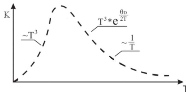
Fig. 1.8. The temperature dependence of the phonon thermal conduction [20].
