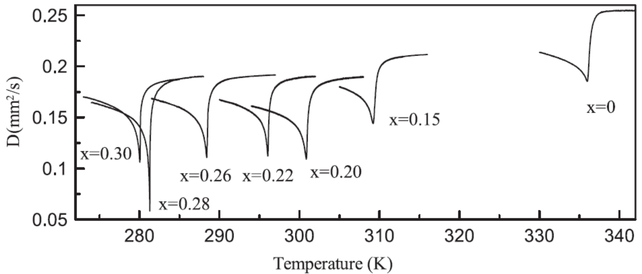
Fig. 8.3. Thermal diffusivity as a function of temperature for the \text{Sn}_2\text{P}_2(\text{S}_{1-x}\text{Se}_x)_6 family near a Lifshitz point [60].
