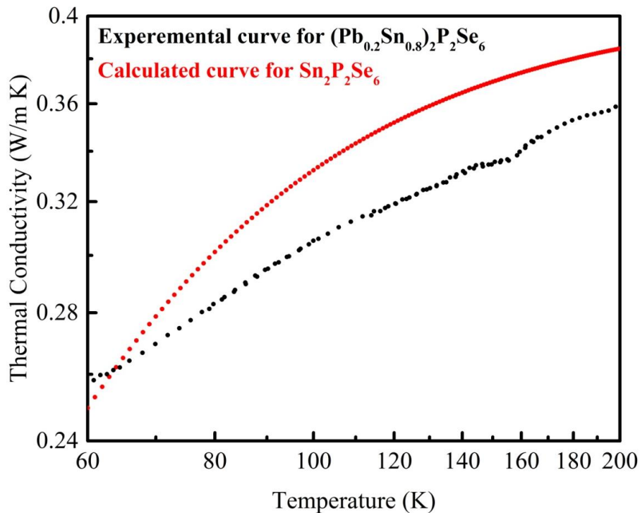
Fig. 9.7. Experimental thermal conductivity curve for (\text{Pb}_{0.2}\text{Sn}_{0.8})_2\text{P}_2\text{Se}_6 (black dots) and minimum calculated value for \text{Sn}_2\text{P}_2\text{Se}_6 using eq. 9.1 (red dots).
