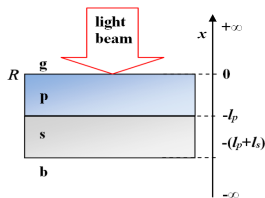
Fig. 2.4. Geometry of the PPE in front-detection configuration with opaque sensor.
