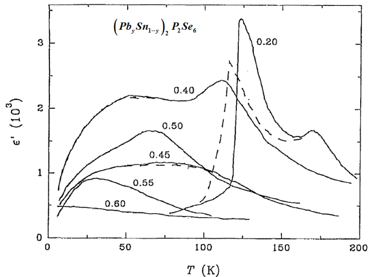
Fig. 3.24. Temperature dependence of the real part of dielectric permittivity for (\text{Sn}_{1-y}\text{Pb}_y)_2\text{P}_2\text{Se}_6 mixed ferroelectrics with different Pb content. Dashed line – cooling, solid line – heating [112].
