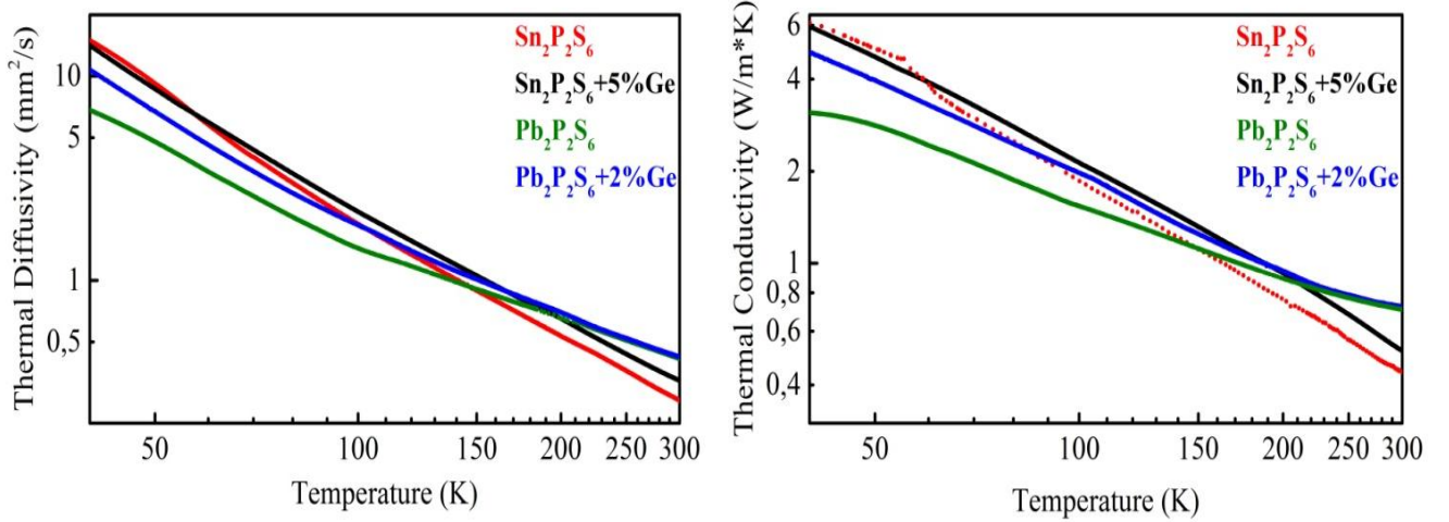
Fig. 9.5. Temperature dependence of thermal diffusivity (left panel) and thermal conductivity (right panel) for nominally pure \text{Pb}_2\text{P}_2\text{S}_6 and \text{Sn}_2\text{P}_2\text{S}_6 crystals in comparison with data for \text{Pb}_2\text{P}_2\text{S}_6 and \text{Sn}_2\text{P}_2\text{S}_6 crystals doped with Ge.
