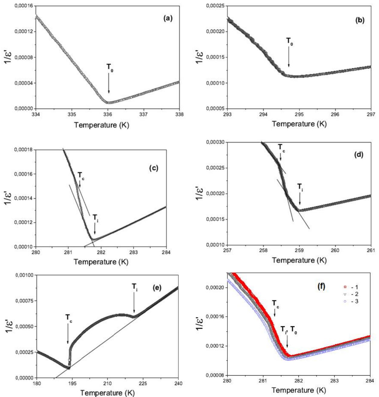
Fig. 3.15. Reciprocal dielectric susceptibility for \text{Sn}_2\text{P}_2(\text{S}_{1-x}\text{Se}_x)_6 ferroelectrics performed at 5mK/min in a cooling regime. (a) – x=0 ; (b) – x=0.22 ; (c) – x=0.28 ; (d) – x=0.40 ; (e) – x=1 ; (f) – x=0.28 at different rates: 0.005K/min (red), 0.05K/min (grey), 0.1K/min (blue) [101].
