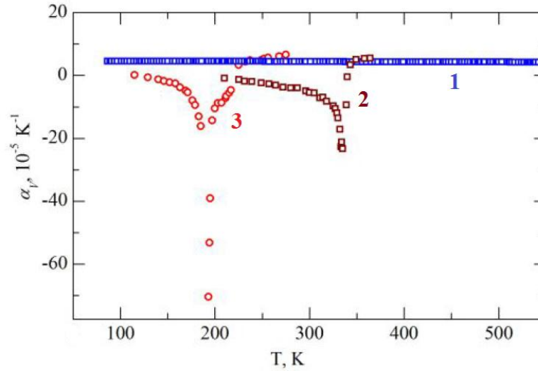
Fig. 3.30. Temperature behavior of the volume thermal expansion coefficient: (1) – \text{Pb}_2\text{P}_2\text{Se}_6 (2) – \text{Sn}_2\text{P}_2\text{S}_6 (3) – \text{Sn}_2\text{P}_2\text{Se}_6 [129].
