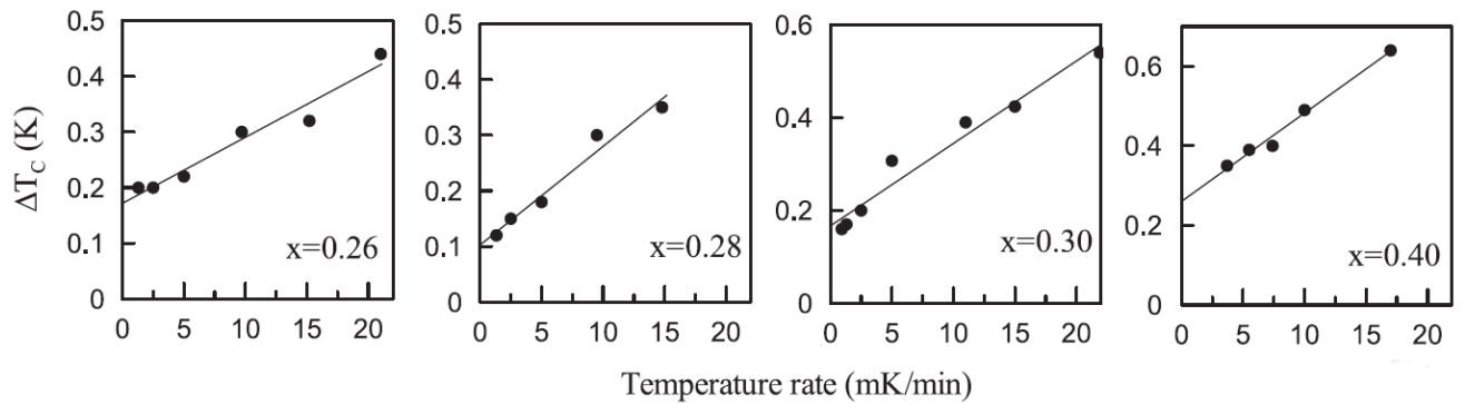
Fig. 8.1. Hysteresis study (difference in the position of the critical temperature in heating and cooling runs as a function of the temperature rate) for \text{Sn}_2\text{P}_2(\text{S}_{1-x}\text{Se}_x)_6 mixed ferroelectrics near the Lifshitz concentration; x=0.28 is the crystal with a Lifshitz point LP [60].
