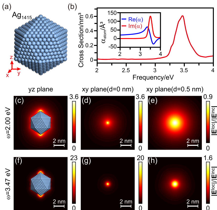
FIGURE 2 (a) Atomistic structure of a \text{Ag}_{1415} nanocluster with a regular icosahedron structure. The orientation is referred to the axis displayed on the bottom-left corner. (b) Absorption spectrum of the nanocluster in (a) for an incident plane wave with electric field polarized along the z -axis, E_z . The inset shows the real and imaginary part of the atomic polarizability of the Ag atoms forming the nanocluster. (c–e) Induced local electric field distribution in the proximity of the nanocluster for an incident optical plane wave with off-resonance energy ( \omega = 2.00 eV) in the (c) yz -plane, in the (d) xy -plane at a distance of d = 0 nm, and in the (e) xy -plane at a distance d = 0.5 nm from the apex of the nanocluster. (f)–(h) show the same local field distributions as in (c)–(e), for incident light in resonance with the nanocluster dipolar mode ( \omega = 3.47 eV)
