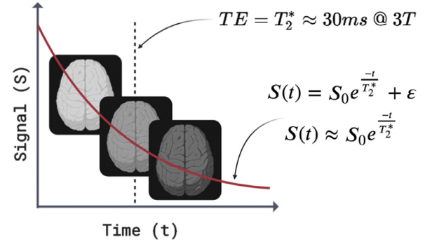
Fig. 1. A representation of mono-exponential signal decay showing diminishing image intensity along three echoes. The second echo is sampled at the optimum echo time equal to average grey matter T_2^* , standard for single echo fMRI. The equation for the red, mono-exponential decay curve is provided (Eq. (1)).
