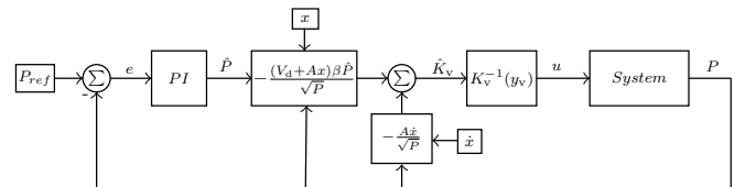
Fig. 2. Force controller block diagram.
