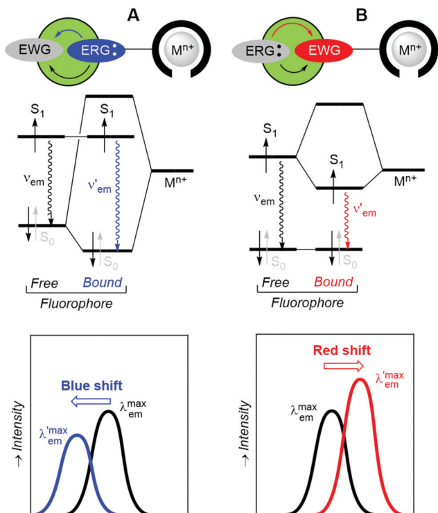
Fig. 3 Schematic representation of intramolecular charge transfer processes (ICT) that modify the fluorescence emission of bicolour sensors in the presence of cations M n+ . (A) Blue shift effect of an electron-releasing group (ERG) close to the ionophore. (B) Red shift effect of an electron-withdrawing group (EWG) close to the ionophore.
