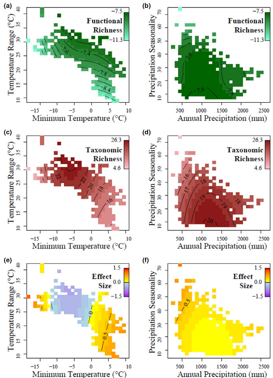
FIGURE 2 Heat maps depicting fitted results of three multiple generalized additive models. Values for functional richness (a + b) indicate the logarithm of the original values, while values for taxonomic richness (c + d) and effect sizes of functional richness (e + f) represent the original values. In panels (a–d), lighter colours indicate lower functional richness values and darker colours indicate higher functional or taxonomic richness values. In panels (e) and (f), yellow to red colours are positive effect sizes, and blue to purple colours are negative effect sizes. White spaces are locations without data and/or represent combinations of climatic variables that do not exist anywhere in Europe
