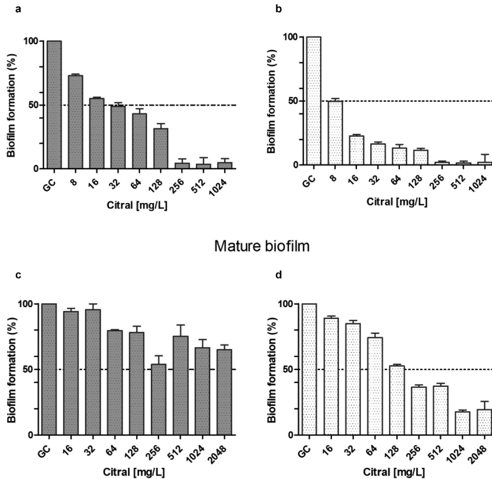
Figure 1. In vitro activity of citral against biofilm by the C. albicans UPV 15–157 azole-resistant isolate. Growth inhibition of the adhesion phase of biofilm-pre-sessile cells by biomass quantification with crystal violet assay (A) and metabolic activity determination with the XTT reduction assay (B). Growth inhibition of mature biofilm-sessile cells by biomass quantification with the crystal violet assay (C) and metabolic activity determination with the XTT reduction assay (D). GC: growth control. The title of figures a and b is missing: Adhesion phase of biofilm. Please add this title or delete the title of figures c and d: Mature biofilm.
