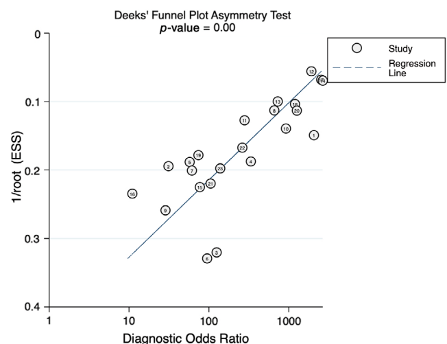
FIGURE 2 Deeks' funnel plot asymmetry test for the diagnostic odds ratio (DOR). The vertical axis displays the inverse of the square root of the effective sample size (1/root[ESS]). The horizontal axis displays the ratio DOR [Color figure can be viewed at wileyonlinelibrary.com ]
