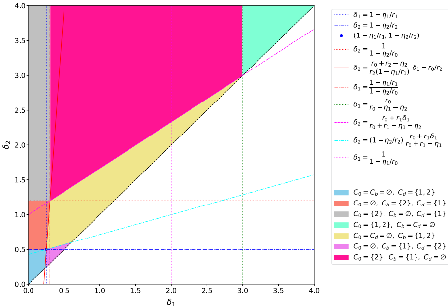
Fig. 2 Conditions 1–7 determine a partition of the half-plane 0 \leq \delta_1 \leq \delta_2
