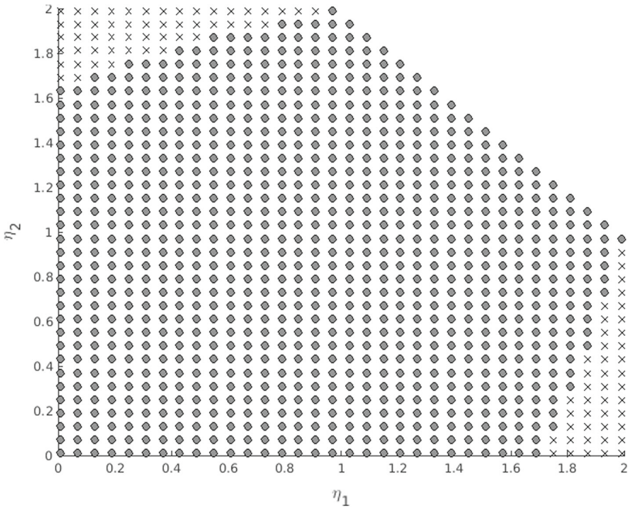
Fig. 3 Comparison of optimal costs of Sect. 5.1 when \delta_i < 1 for i = 1, 2
