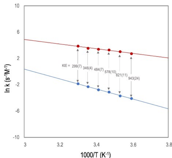
Figure 5. Arrhenius plots for the hydrolysis of \text{Et}_3\text{Si-H} (red) and \text{Et}_3\text{Si-D} (blue) catalyzed by 1 , leading to values of A (from the intercept) and E_{\text{a}} (from the slope). From the differences of the plots the KIE at each temperature is calculated, errors in parenthesis.
