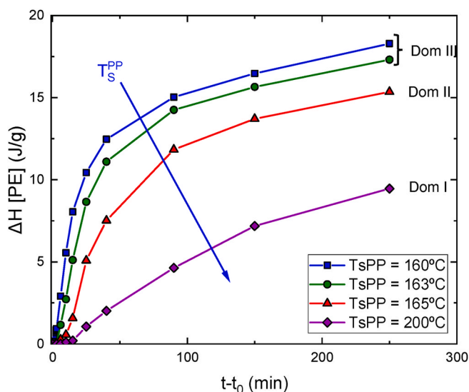
Fig. 10. Melting enthalpy of PE droplets with respect to isothermal time after the self-nucleation protocol for the matrix (PP) phase at different self-nucleation temperatures at a constant PE crystallization temperature of 123^\circ\text{C} for different times.
