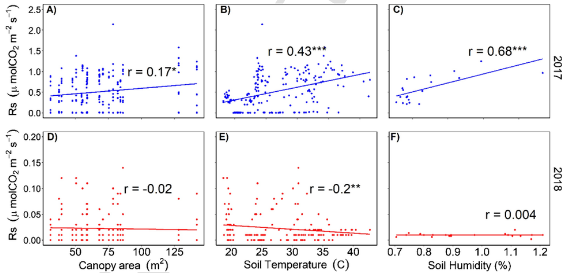
Fig. 3. Pearson correlation analysis between soil respiration and tree canopy area, soil temperature, and soil humidity during 2017 (A, B, and C, respectively, in blue), and during 2018 (D, E, and F, respectively, in red) under the tree canopy. (For interpretation of the references to color in this figure legend, the reader is referred to the web version of this article.)
