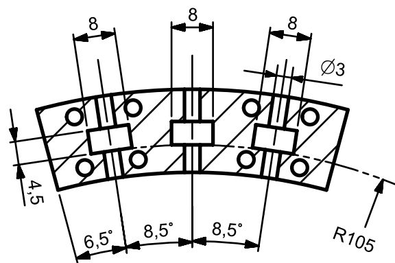
SECTION C-C
