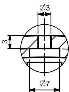
DETAIL D SCALE 2:1
