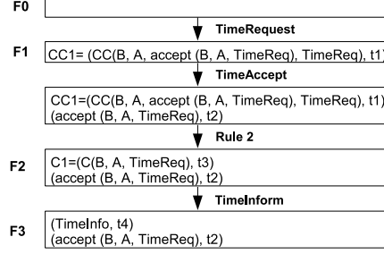
Fig. 2. Protocol fluents
