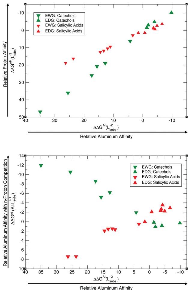
Fig. 9 Proton versus aluminum competition analysed as: (a) \Delta\Delta G^{\text{H}}(\text{L}_{\text{subs}}^{-2}) vs. \Delta\Delta G^{\text{Al}}(\text{L}_{\text{subs}}^{-2}) (top diagram) and (b) \Delta\Delta G^{\text{Al}}(\text{Al-L}_{\text{subs}}^{-2}) vs. \Delta\Delta G^{\text{Al}}(\text{L}_{\text{subs}}^{-2}) (bottom diagram). Terms defined in the body text. All relative affinities are in kcal mol -1 .
