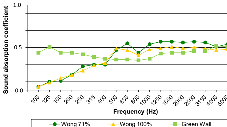
Fig. 11. Sound absorption coefficient value comparison between the green wall and the results reported by Wong et al. [7].
