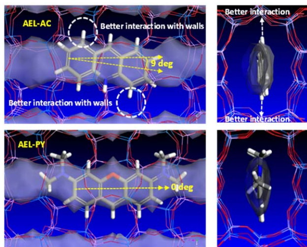
Figure 2. AC (top) and PY (bottom) confined within the AEL channels, and deviation angles; the channel void volume is shown for help of interpretation.
