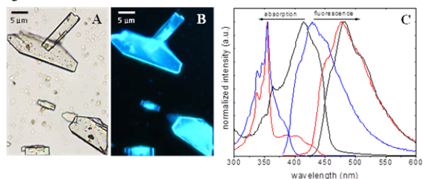
Figure 3. Left) Transmission (A) and fluorescence (B) images under UV illumination (350/50) of AC/AEL crystals; Right) (C) Absorption and fluorescence spectra of Acridine dye in aqueous solution ( 10^{-5} M) at different pHs (red curve: pH < pK_a , blue curve: pH > pK_a ) and bulk powder of AC/AEL (black curve).
