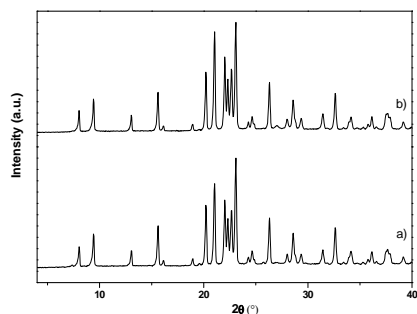
Figure 1. X-ray diffraction pattern of: a) AC/AEL; b) AC-PY/AEL
