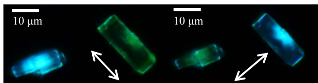
Figure 5. Transmission and polarized intensity fluorescence images of a single particle of AC-PY/AEL for orthogonal polarizations (arrows indicates the direction of the polarized light).
