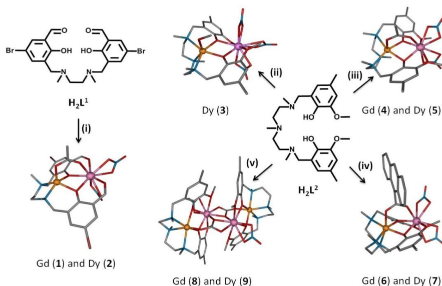
Fig. 1. (i) \text{H}_2\text{L}^1/\text{Mn}(\text{OAc})_2 \cdot 4\text{H}_2\text{O}/\text{Ln}(\text{NO}_3)_3 \cdot n\text{H}_2\text{O} , 1:1:1 in \text{CH}_3\text{CN}/\text{MeOH} (Ln = Gd (1), Dy (2)). (ii) \text{H}_2\text{L}^2/\text{Mn}(\text{NO}_3)_2 \cdot 4\text{H}_2\text{O}/\text{Dy}(\text{NO}_3)_3 \cdot 5\text{H}_2\text{O} , 1:1:1 in MeOH (3). (iii) \text{H}_2\text{L}^2/\text{Mn}(\text{OAc})_2 \cdot 4\text{H}_2\text{O}/\text{Ln}(\text{NO}_3)_3 \cdot n\text{H}_2\text{O} , 1:1:1 in MeOH (Ln = Gd (4), Dy (5)). (iv) \text{H}_2\text{L}^2/\text{Mn}(\text{NO}_3)_2 \cdot 4\text{H}_2\text{O}/\text{Ln}(\text{NO}_3)_3 \cdot n\text{H}_2\text{O}/\text{H}_2\text{-9-An}/\text{Et}_3\text{N} , 1:1:1:1:1 in \text{CH}_3\text{CN} (Ln = Gd (6), Dy (7)). (v) \text{H}_2\text{L}^2/\text{Mn}(\text{NO}_3)_2 \cdot 4\text{H}_2\text{O}/\text{Ln}(\text{NO}_3)_3 \cdot n\text{H}_2\text{O}/\text{Et}_3\text{N}/\text{Na}_2\text{CO}_3 , 1:1:1:2:1 in \text{CH}_3\text{OH}/\text{H}_2\text{O} (Ln = Dy (8), Gd (9)). Hydrogen atoms are omitted for the sake of clarity. Colour code: N = blue, O = red, C = gray, Br = brown, Mn = orange, Ln = pink.
