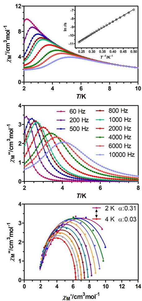
Fig. 8. Temperature dependence of the in-phase \chi_M' (top) and out-of-phase \chi_M'' (middle) components of the ac susceptibility for compound 3 under an external field of 1000 Oe. Inset: Arrhenius plot
