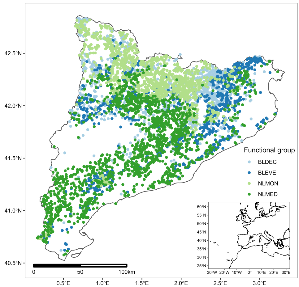
Figure 1. Study area. Map of Catalonia and the forest plots included in the analysis, with colored dots illustrating the functional group of the dominant species of each plot (light blue: BLDEC, broadleaf deciduous, dark blue: BLEVE, broadleaf evergreen, light green: NLMON, needleleaf montane, dark green: NLMED, needleleaf Mediterranean). Inset: the black area represents the location of the study area (Catalonia) within the Western Mediterranean Basin.
