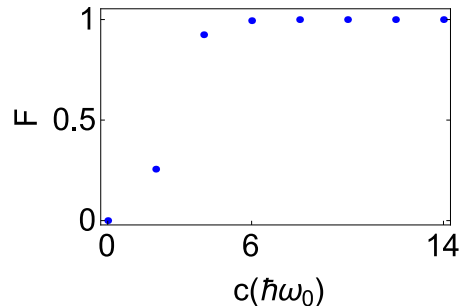
FIG. 5: Fidelity F \equiv |\langle \psi^e(x, t_f) | \psi_f(x) \rangle|^2 versus the potential truncation constant c , where \psi^e(x, t_f) is the final wave function evolved using the truncated potential V_{\text{trun}} . t_f = 8\pi/\omega_0 .
