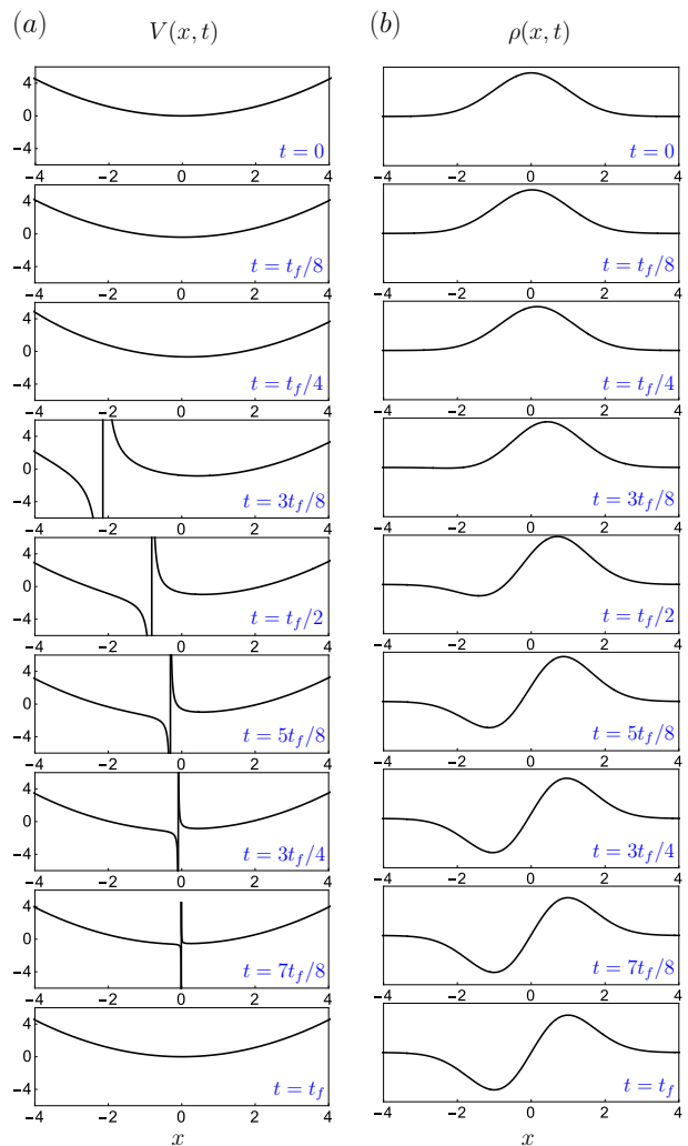
FIG. 4: (a) Snapshots of the time evolution of the trap shape that connects the ground state to the first excited state of a harmonic potential ( \omega_0 = 1 ). The transformation is calculated in a time t_f = 8\pi . (b) \rho(x, t) (in arbitrary units) is plotted as a function of the position in the course of the transformation.
