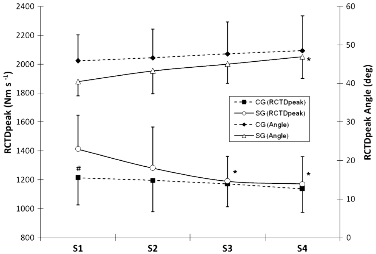
FIGURE 4—Mean values (TSD) of rate of peak crank torque development (RCTDpeak) and angle at RCTDpeak in the relatively stiff (SG) and relatively compliant groups (CG) across the four cycling sprints (S1, S2, S3, and S4). *Significantly different from S1 (P G 0.05). #Significantly different from SG (P G 0.05).
