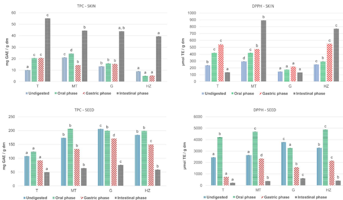
Fig. 1 Changes in total phenolic content (TPC) and antioxidant capacity (DPPH) during in vitro gastrointestinal digestion of different skin and seed grape varieties. *Results are expressed as mean ± standard deviation (n = 3). Different letters in the same stage of the in vitro gastrointestinal digestion represent significant difference among the
