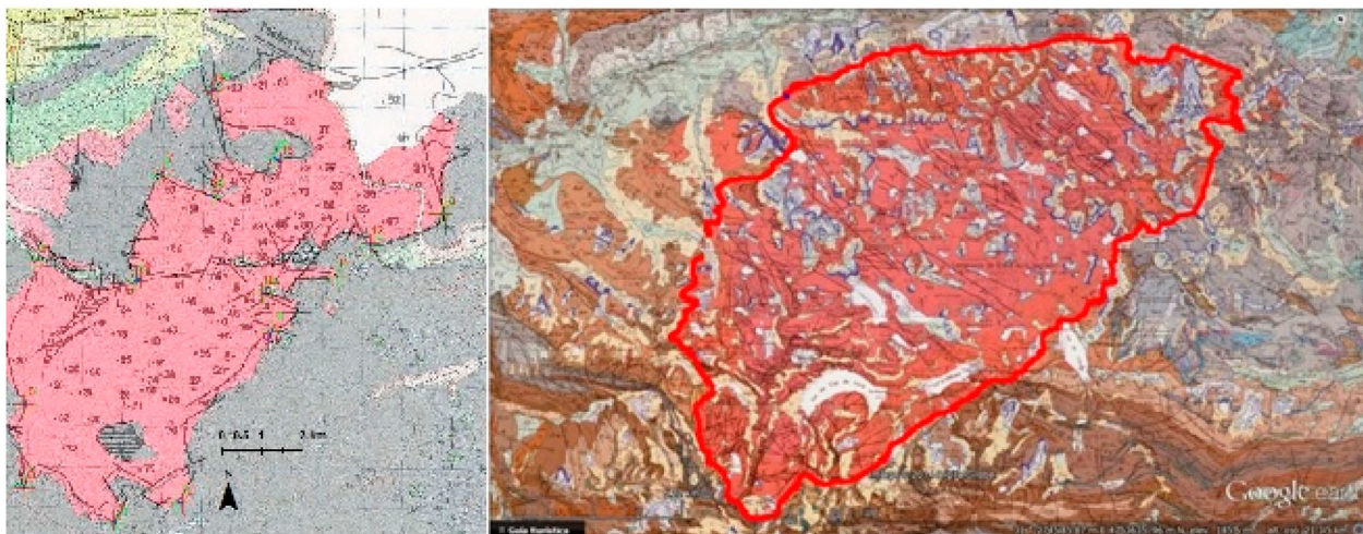
Figure 4. Example of MAGNA (left) and BRGM (on Google Earth, right) maps for the Aya and Neouvelle Plutons. The contact with the host rocks has been highlighted and used as a main marker during the georeferencing process.
