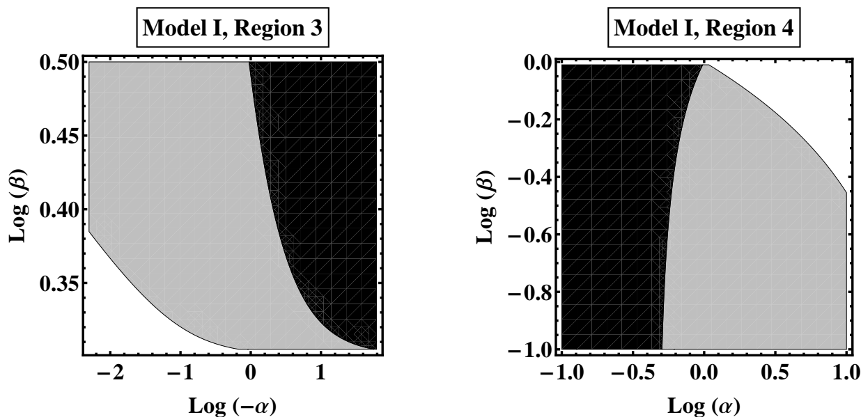
Figure 7. Thermodynamical regions for Model I. We distinguish between three different regions: (i) C < 0 and F > 0 , in black; (ii) C > 0 and F > 0 , in gray; (iii) C > 0 and F < 0 , in white.
