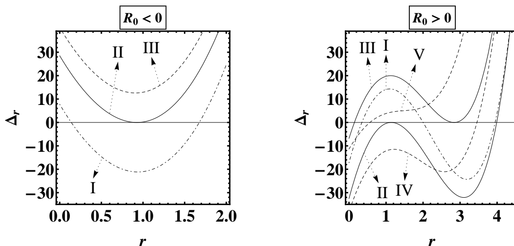
Figure 1. Graphics showing horizons positions as solutions of the equation \Delta_r = 0 taken from [120,121]. On the left panel ( R_0 < 0 ) the presented cases are: h > 0 (I), BH with well-defined horizons, dashed with dots), h = 0 (II), extremal BH, continuous line) and h < 0 (III), naked singularity , dashed). On the right panel ( R_0 > 0 ) the represented cases are: h < 0 (I, BH with well-defined horizons, dashed with dots), h = 0 (II, extremal BH and III, extremal marginal BH, continuous line), and h > 0 (IV, naked singularity and V, naked marginal singularity , dashed).
