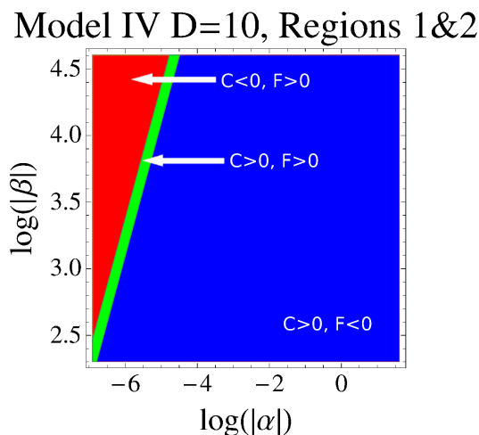
Figure 5. Thermodynamical regions in the (|\alpha|, |\beta|) plane for Model I in D = 10 .
