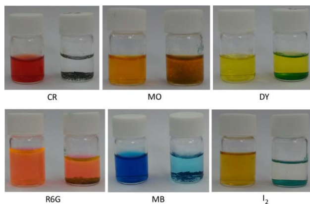
Fig. 2 Color changes of dyes and iodine solutions. All photos were taken after 7 days since the addition of αMOP@Ei2-1 .
