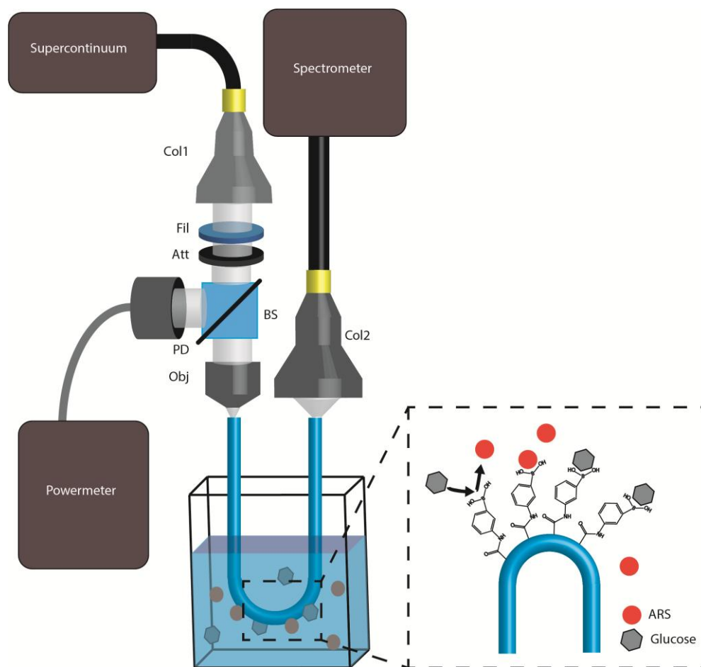
Figure 6. Experimental setup employed to carry out the measurements. Legend: Col1/Col2: collimators, Fil: band-pass filter (390–750 nm), Att: optical attenuator of optical density 3, BS: beam-splitter, Obj: objective, and PD: photo detector; next to the cuvette a chemical illustration of the disaggregation of the ARS is also shown.
