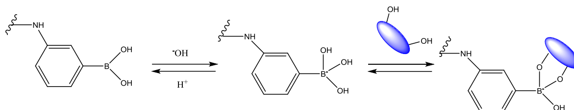
Figure 2. Simplified 3-aminophenylboronic acid (APBA) equilibrium in the presence of glucose.
