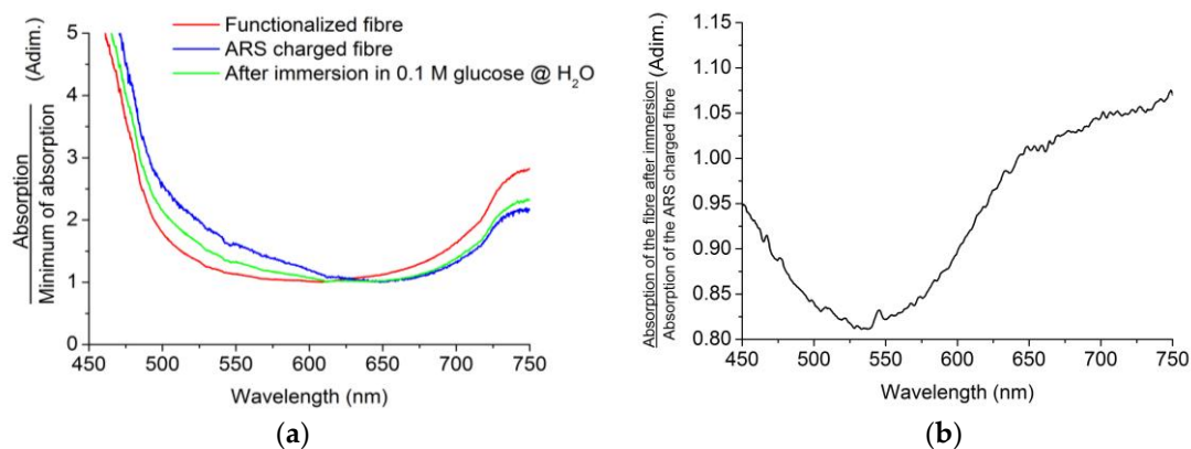
Figure 9. (a) Normalized absorption curves of the probe before and after 10 min of immersion in 0.1 M glucose solution in H_2O ; (b) division of ARS-charged absorption and post-immersion absorption curves.
