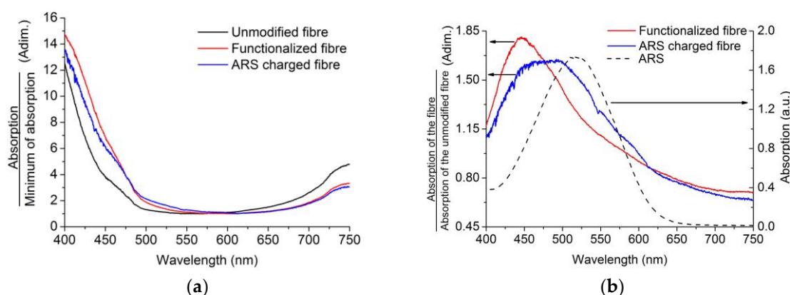
Figure 8. Normalized absorption curves of different probes: (a) unmodified, functionalized, and ARS-charged fibers; (b) absorption curve of functionalized and ARS-charged probe normalized with the unmodified probe and the absorption curve of ARS.
