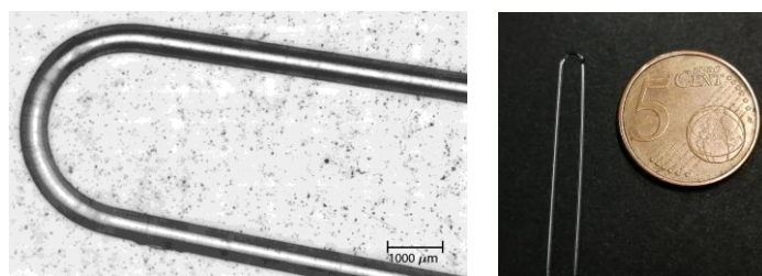
Figure 4. Pictures of the sensor-probe: microscopic picture (left) and a comparison with a 5 cent Euro coin (right).
