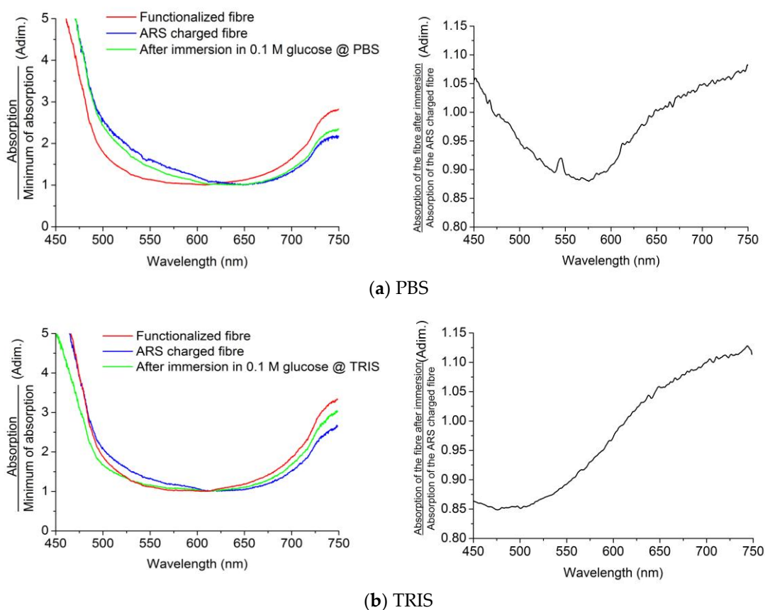
Figure 10. Normalized absorption curves of the probe before and after 10 min of immersion in 0.1 M glucose solution in PBS (a) and TRIS (b) (left); division of ARS-charged absorption and post-immersion absorption curves (right).
