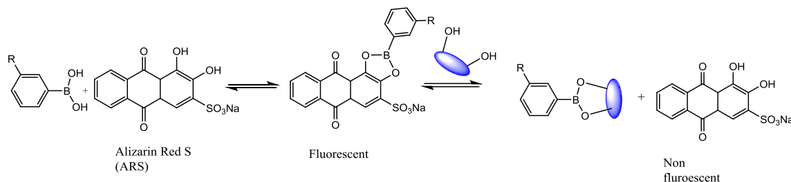
Figure 3. Competitive binding of phenylboronic acid (PBA) with Alizarin Red S (ARS) and glucose.
