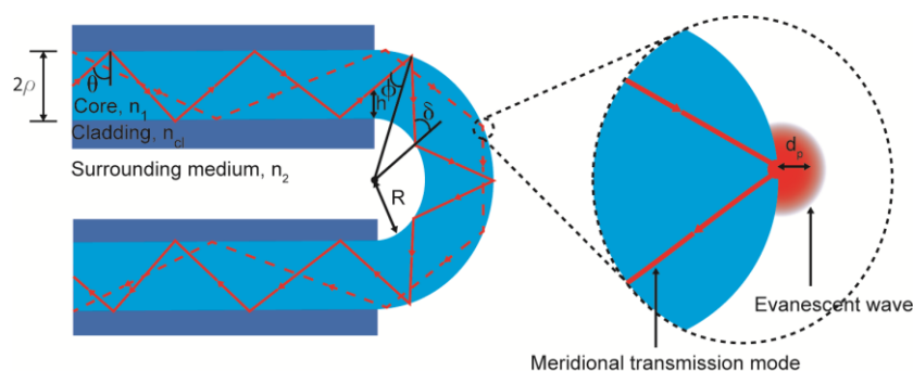
Figure 1. Geometry of the U-shaped sensing region and the representation of a meridional transmission mode (left); illustration of the penetration depth (right).
