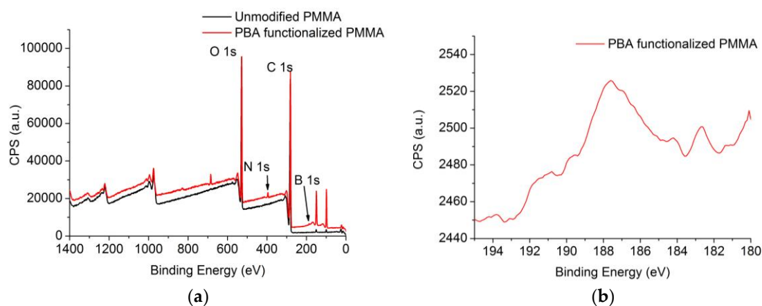
Figure 7. (a) General X-ray photoelectron spectroscopy (XPS) spectra of PBA functionalized and unmodified PMMA plain samples; (b) high resolution spectra of the PBA functionalized sample for boron 1s.
