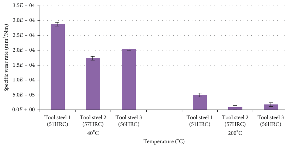
FIGURE 6: Specific wear rate of the pins at 40°C and 200°C.
