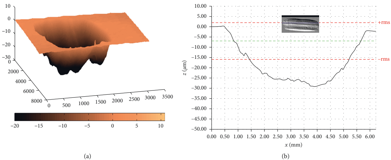
FIGURE 18: Three-dimensional image of the disk track of steel 2 tested at 200°C (a). The maximum profile depth (29 \mu\text{m} ) (b).
