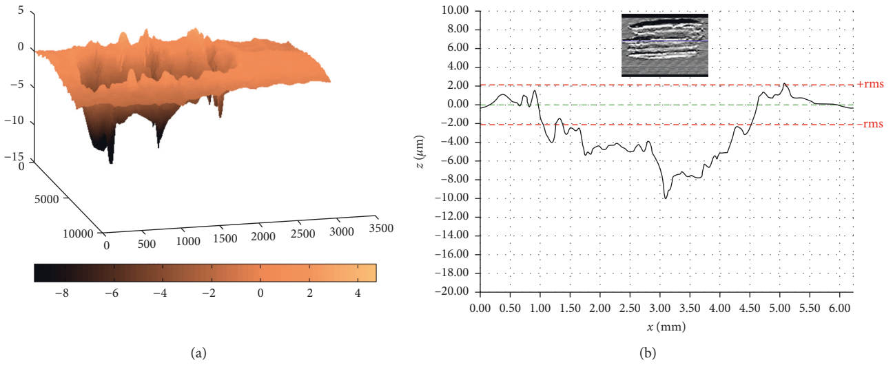
FIGURE 12: Three-dimensional image of the disk track of steel 3 tested at 40°C (a). The maximum profile depth (10 \mu\text{m} ) (b).
