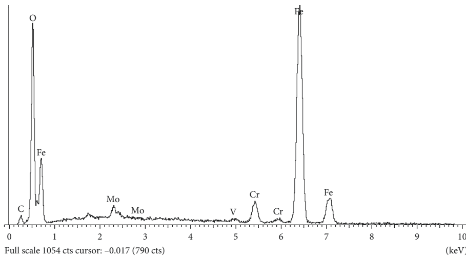
FIGURE 10: EDS spectrum of the oxides in Figure 9.
