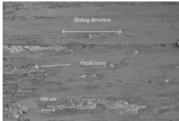
FIGURE 9: Scanning electron microscope micrograph of the steel 3 disk surface tested at 40°C.
