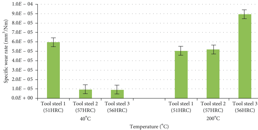
FIGURE 5: Specific wear rate of the disks at 40°C and 200°C.
