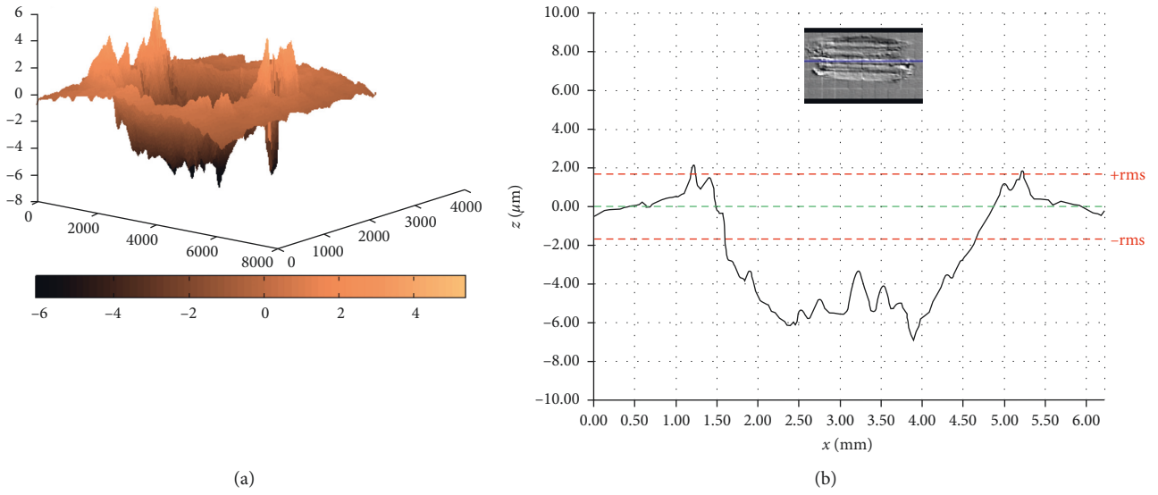
FIGURE 11: Three-dimensional image of the disk track of steel 2 tested at 40°C (a). The maximum profile depth (7 \mu\text{m} ) (b).
