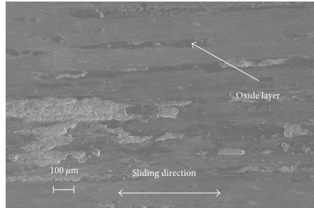
FIGURE 7: Scanning electron microscope micrograph of the steel 2 disk surface tested at 40^\circ\text{C} .
