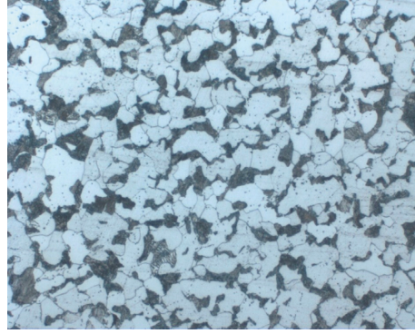
FIGURE 1: Microstructure of the pin is composed of ferrite and pearlite.
