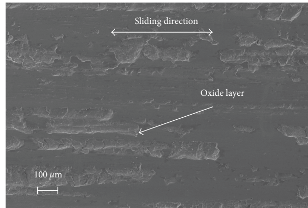
FIGURE 14: Scanning electron microscope micrograph of the steel 1 disk surface tested at 40°C.
