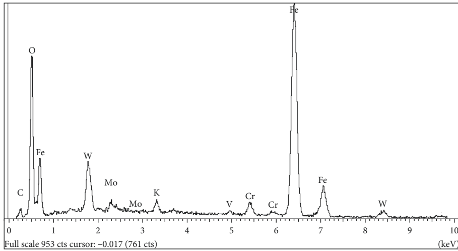
FIGURE 8: EDS spectrum of the oxides in Figure 7.
