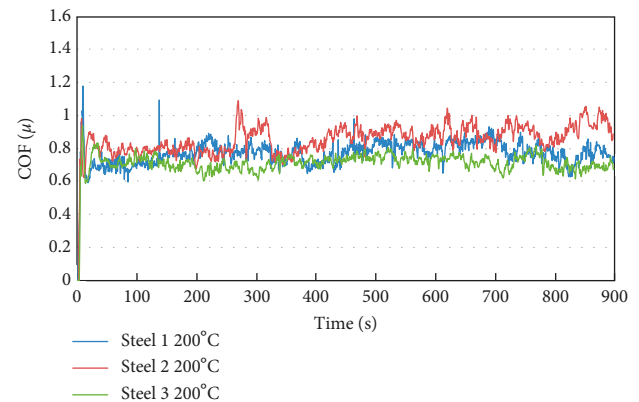
FIGURE 4: COF of the tests performed at 200°C.
