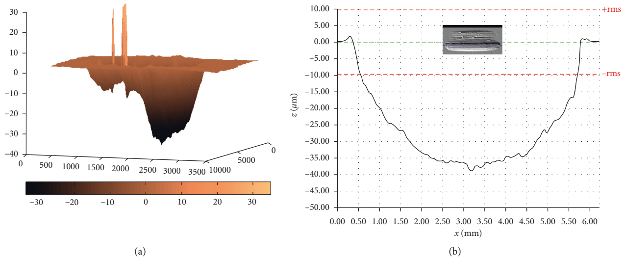
FIGURE 17: Three-dimensional image of the disk track of steel 1 tested at 200°C (a). The maximum profile depth (38 \mu\text{m} ) (b).
