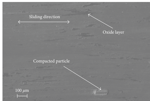
FIGURE 16: Scanning electron microscope micrograph of the steel 2 disk surface tested at 200°C.
