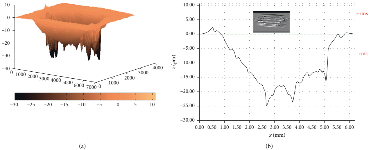
FIGURE 13: Three-dimensional image of the disk track of steel 1 tested at 40°C (a). The maximum profile depth (25 \mu\text{m} ) (b).
