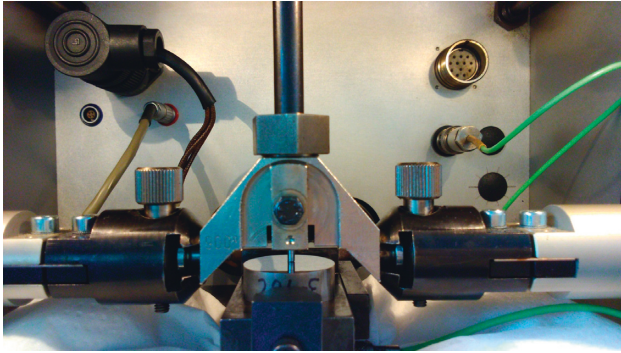
FIGURE 2: Upper and lower specimens in the SRV machine.
