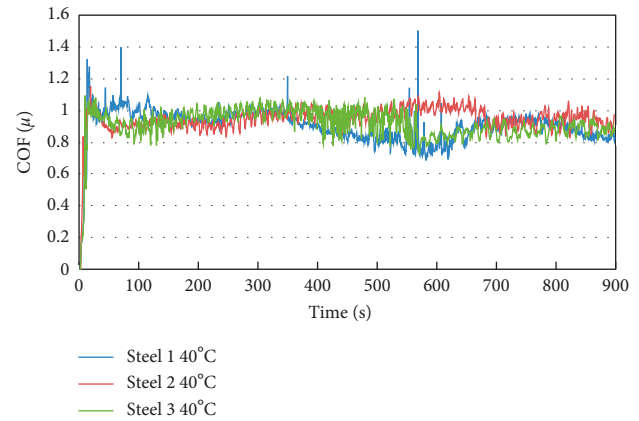
FIGURE 3: COF of the tests performed at 40°C.
