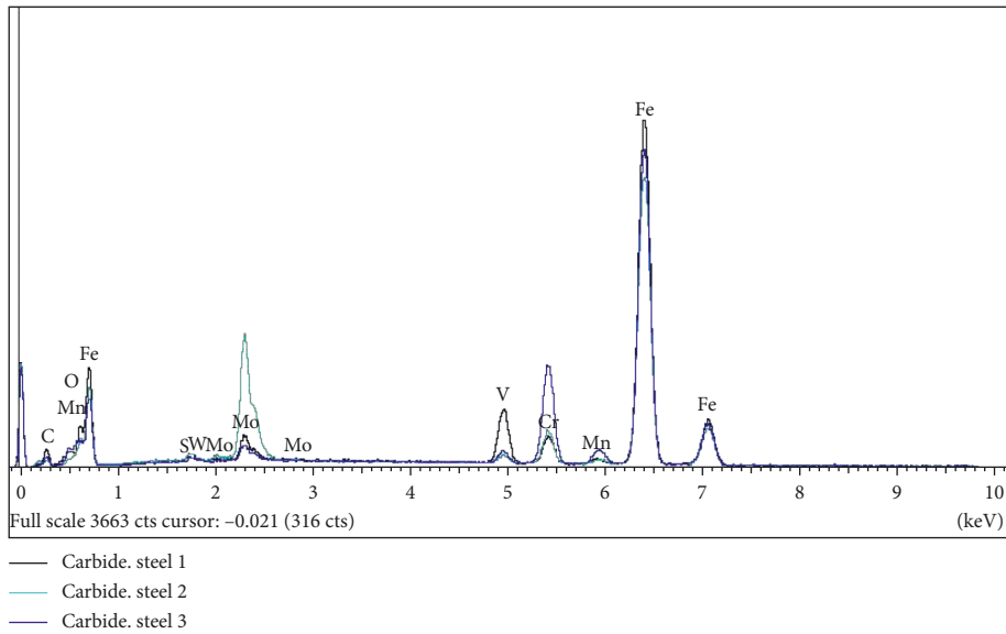
FIGURE 20: Comparison of the carbides' nature of the tool steels studied.
