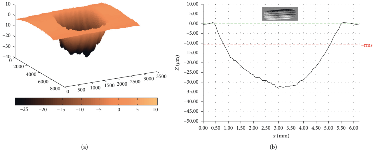
FIGURE 19: Three-dimensional image of the disk track of steel 3 tested at 200°C (a). The maximum profile depth (32 μm) (b).
