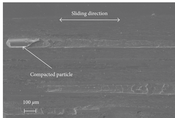
FIGURE 15: Scanning electron microscope micrograph of the steel 1 disk surface tested at 200°C.
