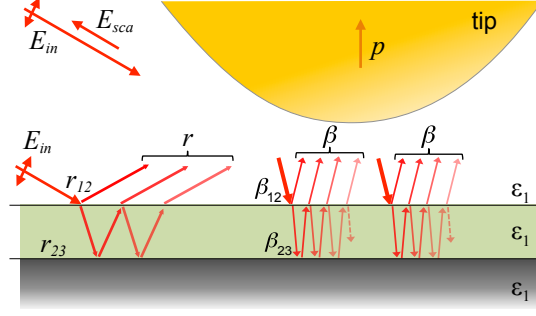
Figure 6.4: Illustration of the far-field illumination of the tip, and of the near-field interaction/scattering between the tip and the sample.
