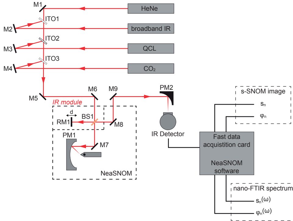
Figure 3.11: IR s-SNOM setup used in this work. The experimental setup comprises a neaSNOm near-field microscope, beamsplitter (BS1), a moving reference mirror (RM1), and a IR detector. As IR light sources are employed a CO 2 laser and a QCL for s-SNOM imaging, and a broadband IR super-continuum for nano-FTIR spectroscopy. A HeNe laser is used for alignment purposes only, several optical components (such as mirrors and windows) are used for guiding and selecting the respective laser beam, and a computer with a fast data acquisition card and the neaSNOm software is used for recording the data.
