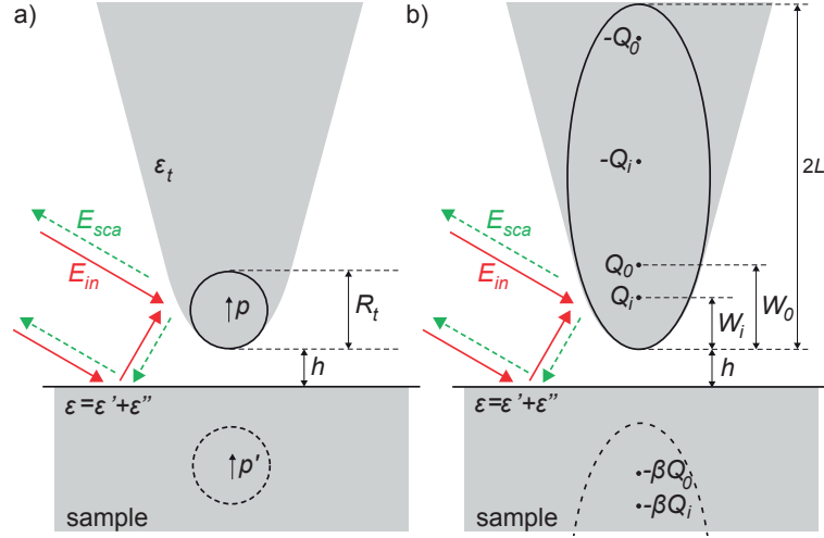
Figure 3.13: Schematics of the a) Point Dipole Model, and b) Finite Dipole Model.
