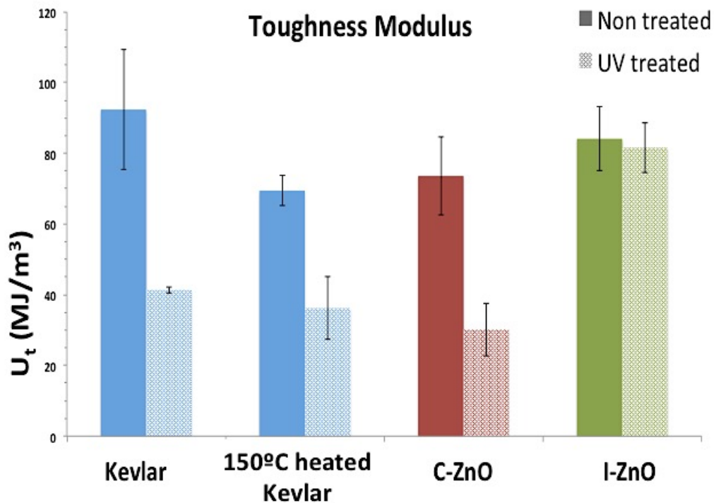
Figure 3.7: Modulus of toughness of the various processed samples before and after UV irradiation.
