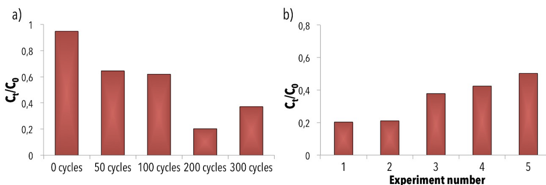
Figure 5.11: The photocatalytic activity of I-ZnO as a function of a) the number of infiltration cycles and b) the number of consecutive experiments (200 cycles sample).
