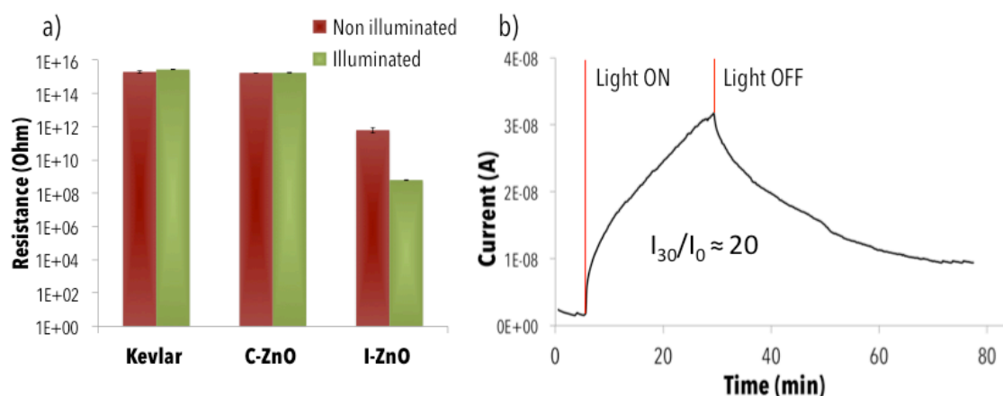
Figure 5.9: a) Comparison of electrical resistance of untreated, C-ZnO and I-ZnO Kevlar fibres in the dark and when illuminated with visible light. All samples were measured after bending. b) Photocurrent measurement of I-ZnO Kevlar fibres under visible light applying a bias voltage of 10V.
