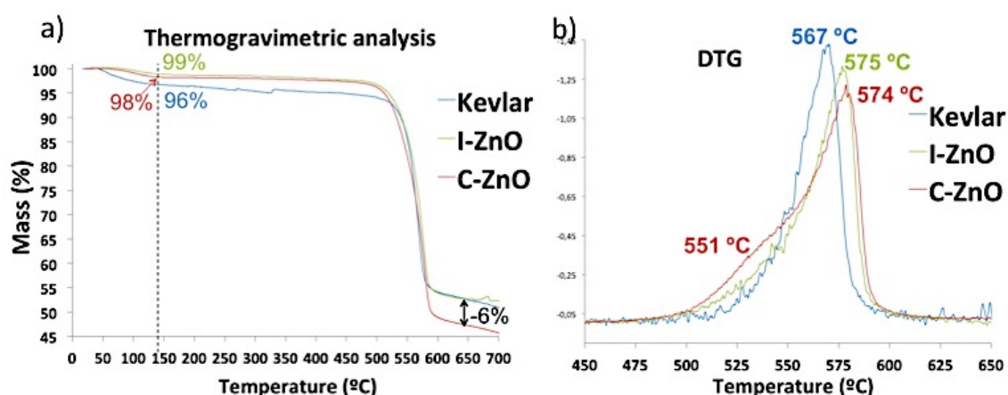
Figure 3.5: a) Thermogravimetric analyses showing the mass loss of each sample as a function of temperature, b) Derivative thermogravimetric plots showing the main degradation temperature of each sample. The temperature values of the C-ZnO sample correspond to the maxima of the deconvoluted peaks.
