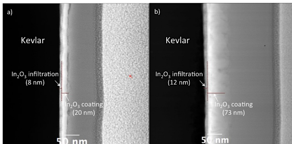
Figure 5.8: TEM images of the cross-sectioned area of the 700 cycles I-In 2 O 3 Kevlar fibres after following exposure times: a) 10 s and b) 90 s.
