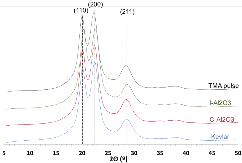
Figure 4.3: XRD diffraction patterns of the samples.
