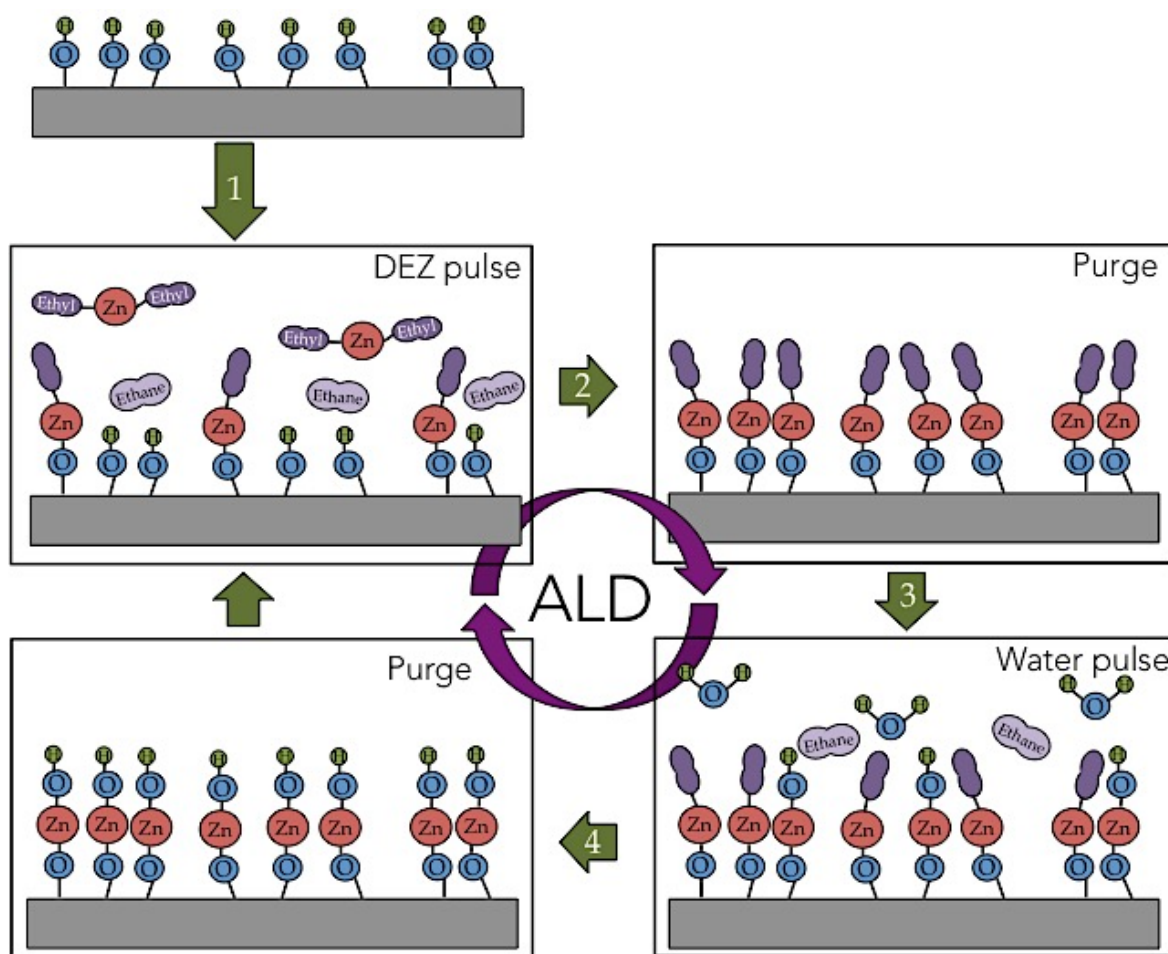
Figure 1.3: Schematic of the ALD deposition of ZnO using diethylzinc and water as precursors.
