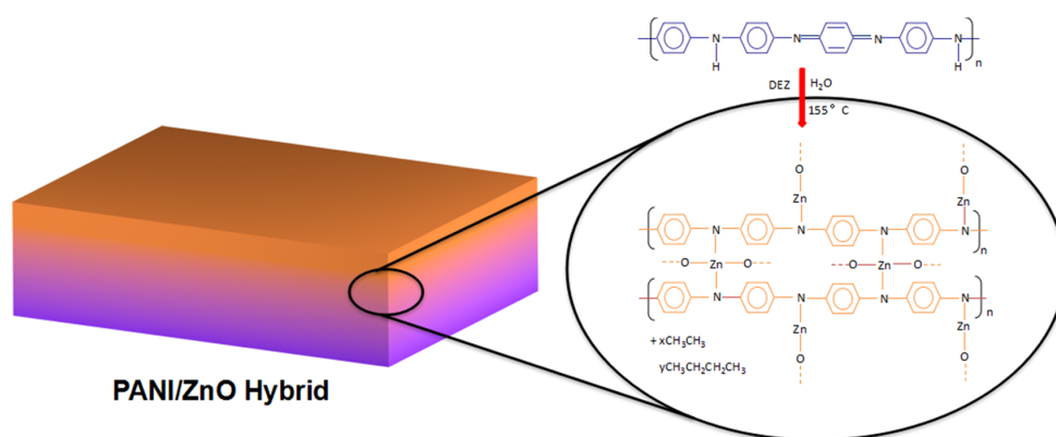
Figure 1.5: Schematic of a PANI substrate after doping with ZnO by VPI. The ZnO cross-links the polymer chains oxidizing the polymer backbone and at the same time becomes doped through the N from PANI. In this way, both components, the PANI and ZnO synergistically contribute to the conductivity of the hybrid. Reprinted with permission from 72 . Copyright 2017 American Chemical Society.
