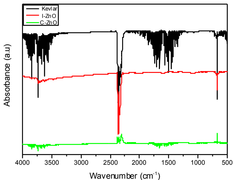
Figure 3.6: FTIR spectra of the evolving gases upon decomposition at 520 °C. In the case of untreated and I-ZnO samples, the absorbance is negative as no gases are released.
