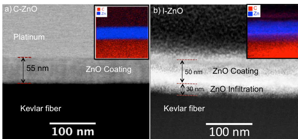
Figure 3.1: TEM images of cross-sections of a) C-ZnO and b) I-ZnO fibres. Insets show EDS colour maps with the carbon signal coded red and the zinc signal coded blue.
