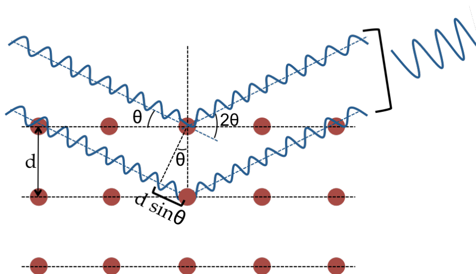
Figure 2.2: Schematic of the principle of XRD, showing the interaction of an X-ray beam with a crystal. When the Bragg's condition is fulfilled, constructive interferences create a reflected peak characteristic of the crystalline material.
