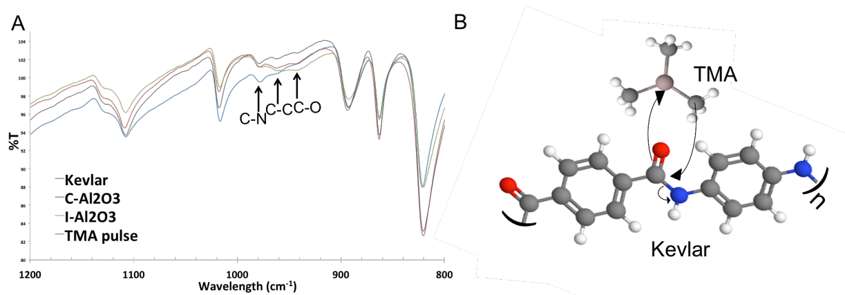
Figure 4.2: A) Fingerprint area ( 1200\text{-}800\text{ cm}^{-1} ) of the ATR-FTIR spectra of Kevlar fibres before and after coating and infiltration. B) Schematic view of the proposed reaction mechanism between Kevlar and TMA, based on the FTIR data.
