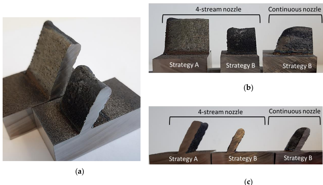
Figure 15. Walls at 30^\circ : (a) comparison of walls fabricated with Strategy A and Strategy B and the four-stream nozzle; (b) distortions in the edges of the walls; (c) cross-section at different conditions.
