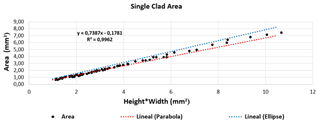
Figure 9. Comparison of the clad areas, using a continuous nozzle with the area of a second-degree parabola ( Area = 2 \cdot (Height \cdot Width) / 3 ) and an ellipse ( Area = \Pi \cdot (Height \cdot Width) / 4 ).
