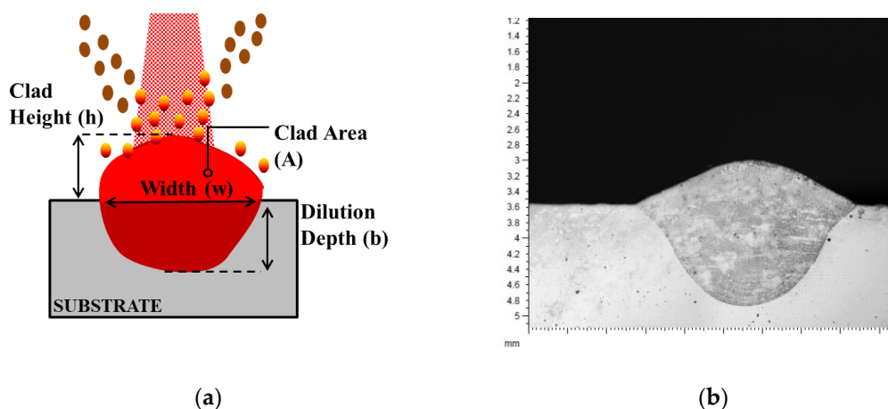
Figure 2. (a) Characteristics of a single clad; (b) macrophotography of a cross-section.
