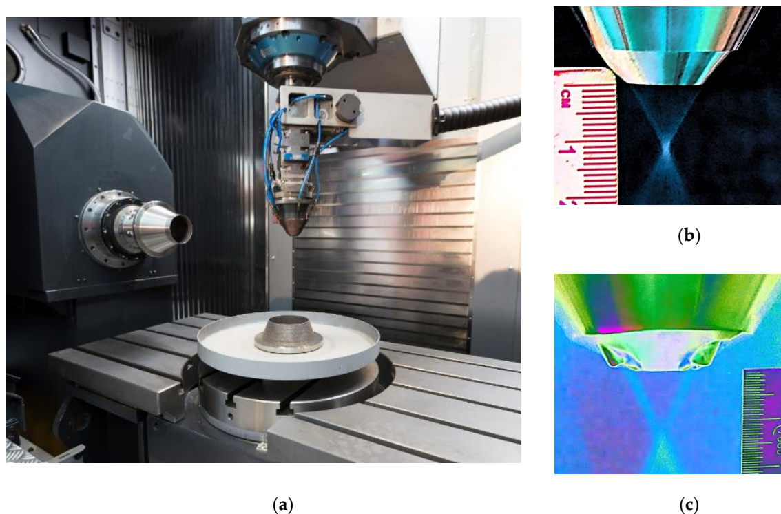
Figure 1. (a) IBARMIA ZVH45/1600 Add+Process hybrid machine; (b) continuous coaxial nozzle with a 0.5 mm slit; (c) 4-stream discrete coaxial nozzle.
