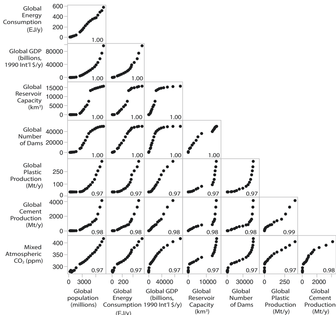
Fig. 4 Statistical relationships between human population, productivity, and energy, and key environmental indicators. Correlation-matrix displayed as cross plots for examples of Late Holocene and Anthropocene environmental factors, including ensemble estimates of global human population (millions), global human energy consumption (EJ/y), global GDP (billions, 1990 Int'l $/y), global reservoir capacity (km 3 ; year-end), global number of large dams (year-end), global plastic production (year-end), global cement production (year-end), mixed atmospheric CO 2 (mid-year). The value in the lower right corner of each plot identifies the Spearman's rank-order correlation coefficients. Data references are listed within Supplementary Online Material.
