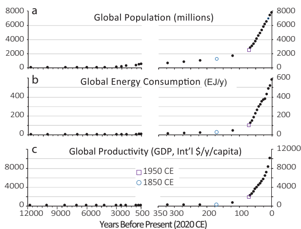
Fig. 1 Correlation of global human population, energy consumption and productivity during the Holocene and Anthropocene epochs. a Global human population (millions), b global energy consumption (EJ/y), and c global productivity ( \$/\text{y}/\text{capita} ), across the Holocene and proposed Anthropocene epochs (in this paper starting in 1950 CE). All three parameters are highly correlated (Spearman's rank coefficient = 1.00). Larger circle = 1850 CE; large square = 1950 CE. Data references are listed in Supplementary Online Material.
