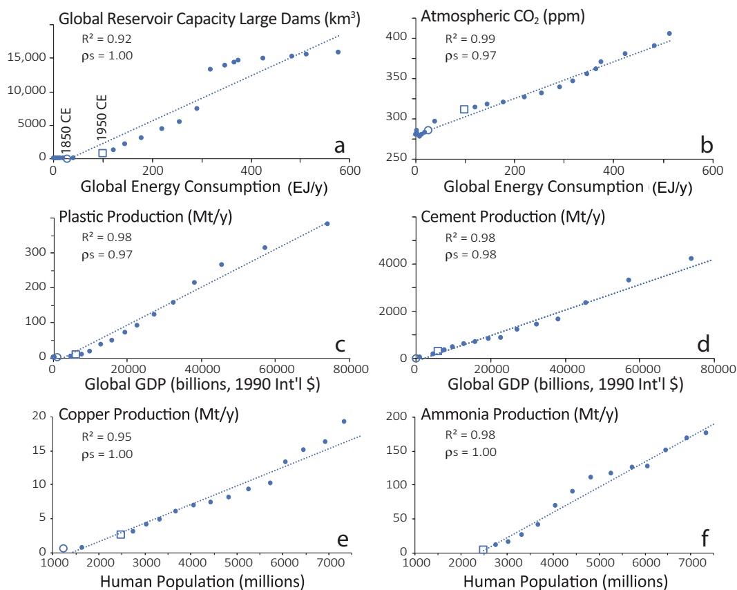
Fig. 3 Global relationships between population, productivity, and energy, the forces behind changes in the environment, and key environmental indicators. Example relationships between the global population (millions), global productivity, and global energy, the forces behind changes in the global environment, and key environmental indicators: a global reservoir capacity of large dams (km 3 ), b mixed atmospheric CO 2 (ppm), c global plastic production (Mt/y), d global cement production (Mt/y), e world copper production (Mt/y), and f world ammonia production (Mt/y) (see Supplementary-Table 2 for data, and Table 2 for other examples). 1850 CE (round) and 1950 CE (square) data points are highlighted. For data references see Supplementary Online Material. Correlation coefficients are provided for both dependent linear relationships (R 2 ) and Spearman’s Rank (ρ s ).
