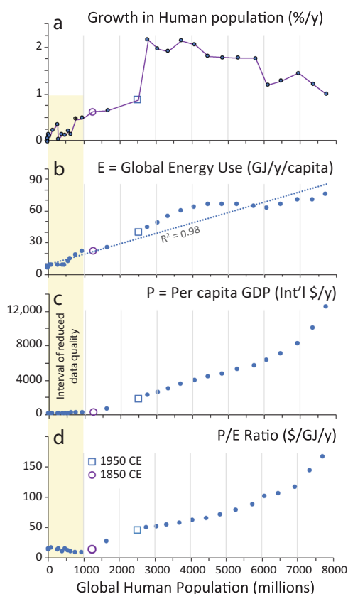
Fig. 2 Relationships between human population (millions) and key economic indicators. Relationships between human population (millions) and key economic indicators: a rate of population growth (%/y), b energy consumption per capita ( E in GJ/y/capita), c per capita productivity ( P as GDP in 1990 international dollars, $/y/capita), and d P/E ratio, each across Holocene and Anthropocene epochs. Purple circle = 1850 CE; blue square = 1950 CE. A marked change in GDP per capita after 1850 CE reflects the global spread of industrialization and technology. The rate of change in population sharply increases around 1950 CE. The P/E ratio fell for most of the Holocene, until 1850 CE, when human society became more productive per unit energy use. Data references are listed in Supplementary Online Material.
